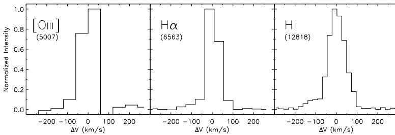
Figure 5.5 – A sample of the narrow emission lines present in the X-shooter spectra: [O III] ( left ) at 5007 Å, Hα ( middle ) and H I (Paβ, right ) at 12818 Å.
