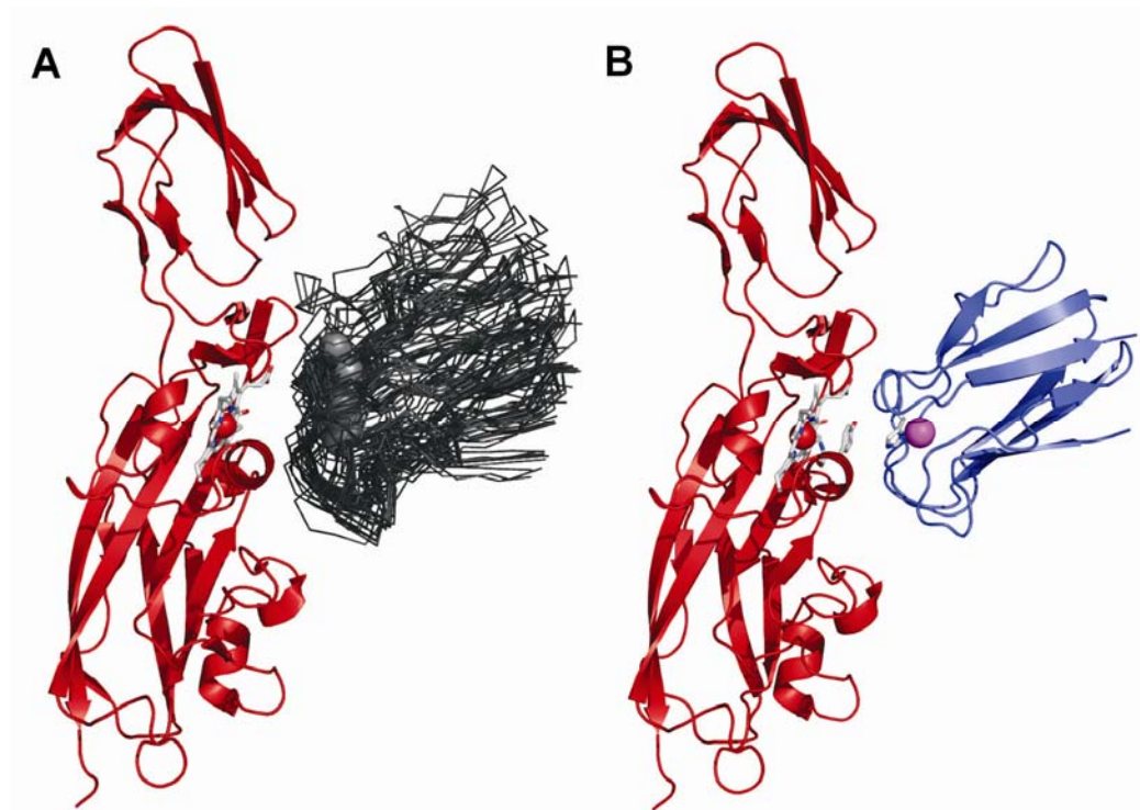
Figure 3.5. Structure of P. hollandica Pc – cytf complex. A) Superposition of the 20 lowest energy conformers. Cyt f is shown as a red ribbon, the haem as sticks and the Fe ion as a sphere; the backbone of Pc is shown as a black C \alpha trace, with the copper ion as a grey sphere. B) Lowest energy representation, Pc is shown as a blue ribbon, with the Cu ion in magenta. Copper ligand His85 and haem ligand Tyr1 are shown as sticks.
