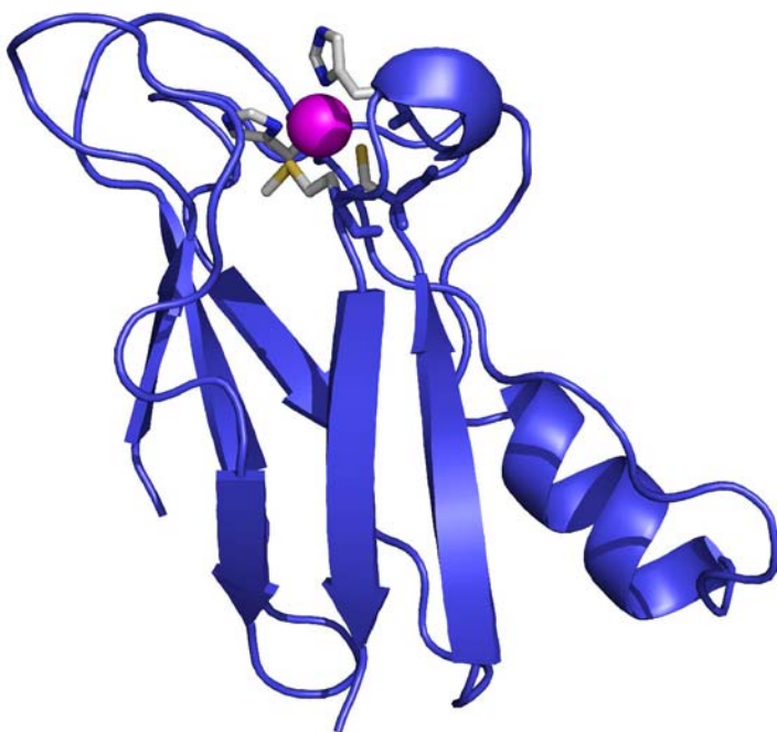
Figure 1.3. Three-dimensional representation of Pc. Pc is shown as a blue ribbon, with the Cu ion as a magenta sphere. The four copper ligands, a cysteine, methionine and two histidines, are shown as sticks. The molecular coordinates were taken from the crystal structure of reduced fern Pc (PDB entry 1KDI). This figure and Figures 1.4, 3.3, 3.5, 3.8, 4.1, 4.4, 4.6 and 5.3 were made in PyMOL v0.98 64 .
