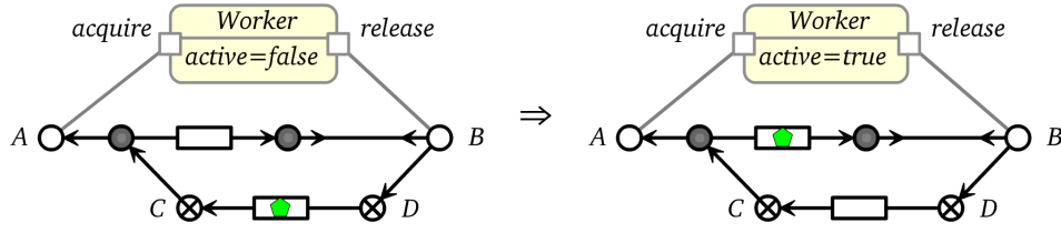
Figure 5.7: execution rule StartWorker
