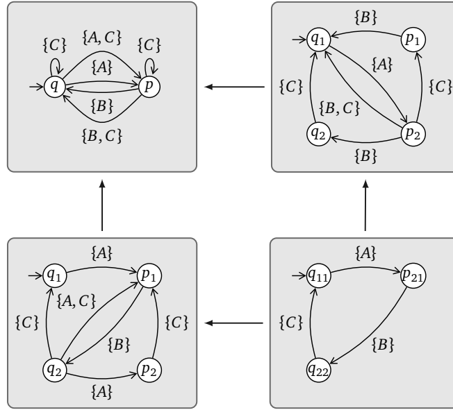
Figure 7.2: a pullback of port automata
