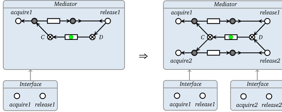
Figure 6.2: example morphism / transformation rule p_1 of distributed Reo graphs
