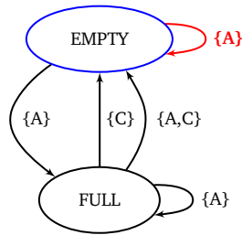
Figure 4.7: non-deterministic (left) vs. context-dependent (right) LossyFIFO in Vereofy
