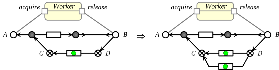
Figure 5.4: reconfiguration rule AddResource
