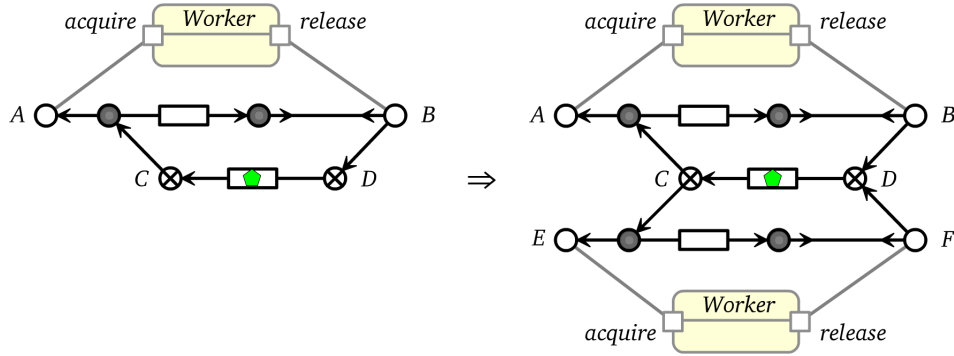
Figure 5.3: reconfiguration rule AddWorker
