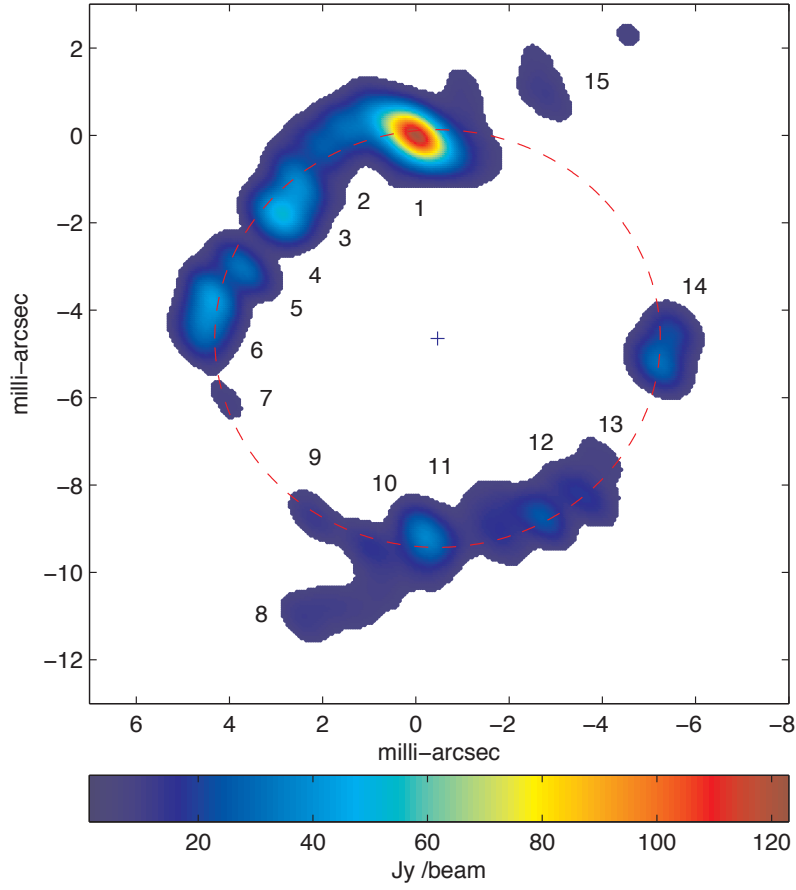
Figure 6.4 – The VLBA map of \nu=1, J=1 \rightarrow 0 SiO maser emission towards the OH/IR star OH 44.8-2.3. The features are color coded according to the flux density (Jy / beam) integrated over all velocity channels.
