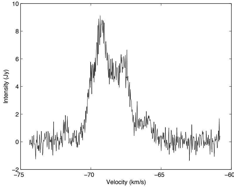
Figure 6.3 – The total intensity spectrum of OH 44.8-2.3 for the v=1, J = 1 \rightarrow 0 SiO maser emission obtained with the VLBA.
