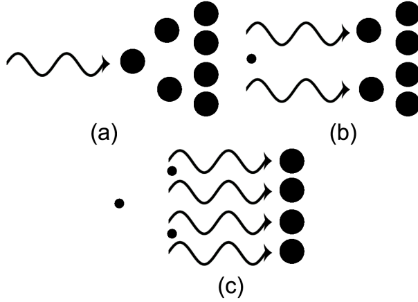
Figure 1.4 – Principle of maser emission: In all frames, the large circles show molecules excited to the upper energy state by a pump. The small circles indicate the molecules in the low energy state. 'a' panel: the molecule in the excited energy state is stimulated by a photon of wavelength \lambda . 'b' panel: The molecule absorbs the photon and re-emits two photons instead to return to the low energy state. These two photons hit the next two excited molecules, which results in 4 photons (panel 'c'). This process continues and as the radiation propagates through the medium, the maser amplifies the radiation exponentially at wavelength \lambda , as long as it is unsaturated.
