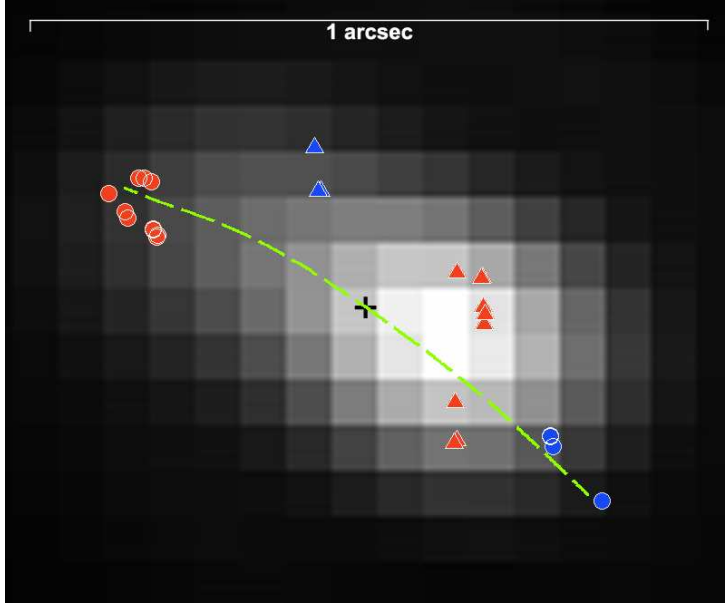
Figure 1.6 – The 12.8\ \mu\text{m} dust image of W43A obtained with the Very Large Telescope (VLT) spectrometer and imager for the mid-infrared (VISIR, Lagadec et al. 2011). The overlaid circles and triangles show the \text{H}_2\text{O} and OH maser features of this star. The dashed line shows the direction of the precessing \text{H}_2\text{O} maser jet.
