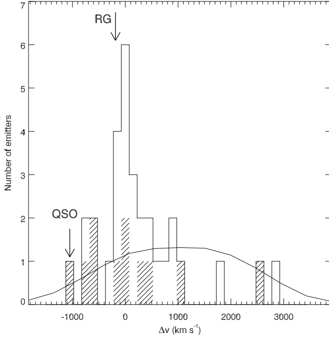
Figure 3.18 — Velocity distribution of the confirmed \text{Ly}\alpha emitters. The bin size is 150 \text{ km s}^{-1} . The median redshift of the confirmed emitters z = 3.1313 is taken as the zero-point. The velocities of the radio galaxy and the QSO are indicated with arrows. The solid line represents the selection function of the narrow-band filter, normalized to the total number of emitters found. The hashed histogram represents the velocities of emitters with absorption in their line profile. The three objects in the red part of the filter (with a velocity greater than 1500 \text{ km s}^{-1} ) might not be part of the protocluster.
