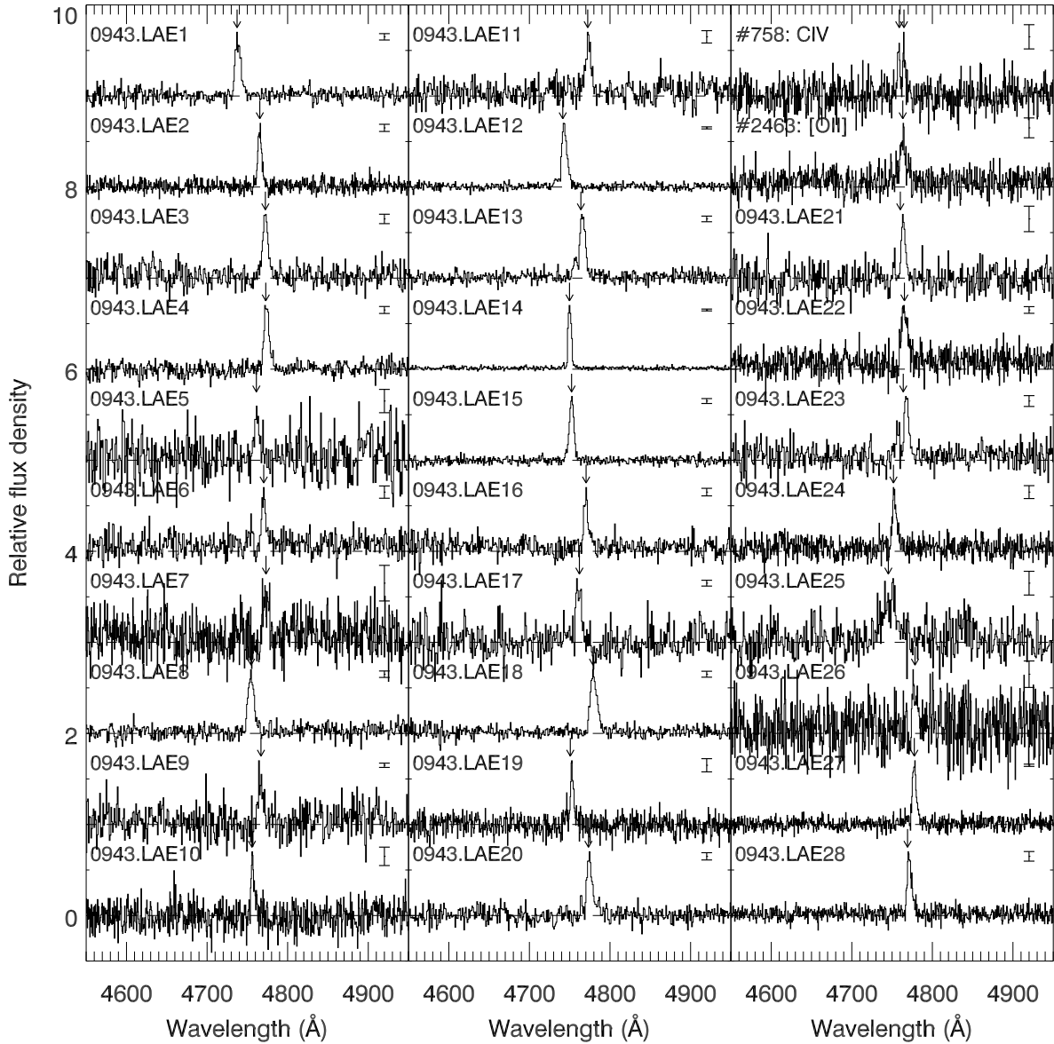
Figure 5.5 — Spectra of the confirmed emitters near the radio galaxy MRC 0943–242. Error bars are shown on the right of each spectrum. All spectra are normalized to the peak of the \text{Ly}\alpha line at a relative flux of 0.7. The offset between the spectra is 1.0. The arrow indicates the redshift of the emitters. The redshift, flux and width of the emission lines can be found in Table 5.8.
