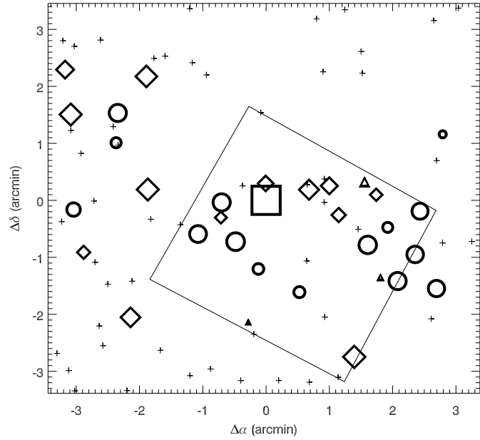
Figure 3.19 — Spatial distribution of \text{Ly}\alpha emitters around the radio galaxy MRC 0316–257 (denoted by a square). The confirmed emitters in the protocluster are represented by circles (emitters with a redshift smaller than the median, z < 3.1313 ) and diamonds (emitters with z > 3.1313 ). The triangles show the position of the three \text{Ly}\alpha emitting galaxies with a velocity > 1500 \text{ km s}^{-1} from the median velocity of the emitters. The sizes of the symbols are scaled according to the velocity offset from the median, with larger symbols representing emitters with a redshift closer to the median redshift. The pluses are objects satisfying the selection criteria (see §3.3.3), but are not (yet) confirmed. The quadrangle represents the outline of the ACS image.
