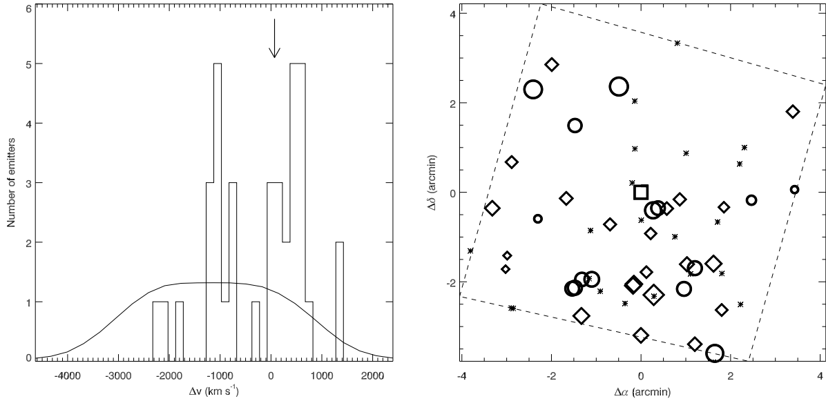
Figure 5.4 — Left: Velocity distribution of the confirmed emitters near MRC 0052-241. The median of the emitters is taken as zero point. The bin size is 150 \text{ km s}^{-1} . The velocity of the radio galaxy is indicated by an arrow. The solid line represents the selection function of the narrow-band filter, normalized to the total number of confirmed emitters. Right: Spatial distribution of the confirmed (circles and diamonds) and candidate (stars) \text{Ly}\alpha emitters. The dashed quadrangle represents the outline of the imaging area. The radio galaxy is denoted by a square. The circles represent the emitters with a redshift smaller than the median redshift ( z < 2.8600 ) and the diamonds the ones with z > 2.8600 . The size of the symbols are scaled according to the velocity offset from the median, with smaller symbols standing for emitters with a redshift farther from the median.
