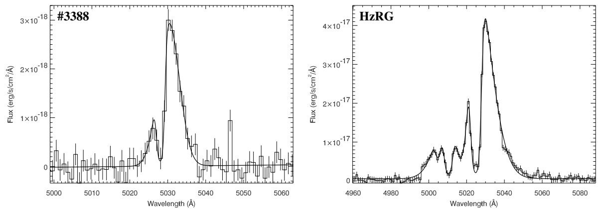
Figure 3.11 — Spectra of emitter #3388 (left) and HzRG (right).
