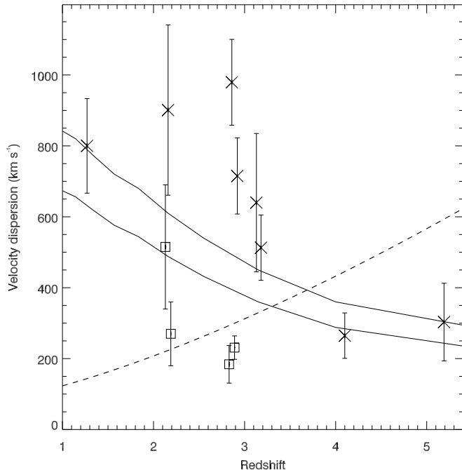
Figure 5.16 — Velocity dispersion of \text{Ly}\alpha emitters in our radio galaxy fields ( crosses ) as a function of redshift. The squares represent the velocity dispersions of the subgroups in the 1138 and 0052 fields (see §5.5.2). The data point near z = 1 represents the velocity dispersion in the X-ray cluster RDCS 1252.9-2927 at z = 1.24 (Rosati et al. 2004). The dashed line is the Hubble flow H(z) over 1 Mpc. The solid lines show the evolution of the dark matter velocity dispersions \sigma_{\text{dm}} of simulated massive clusters (Eke et al. 1998). The top line is scaled to 1000 \text{ km s}^{-1} at z = 0 , the bottom line to 800 \text{ km s}^{-1} at z = 0 .
