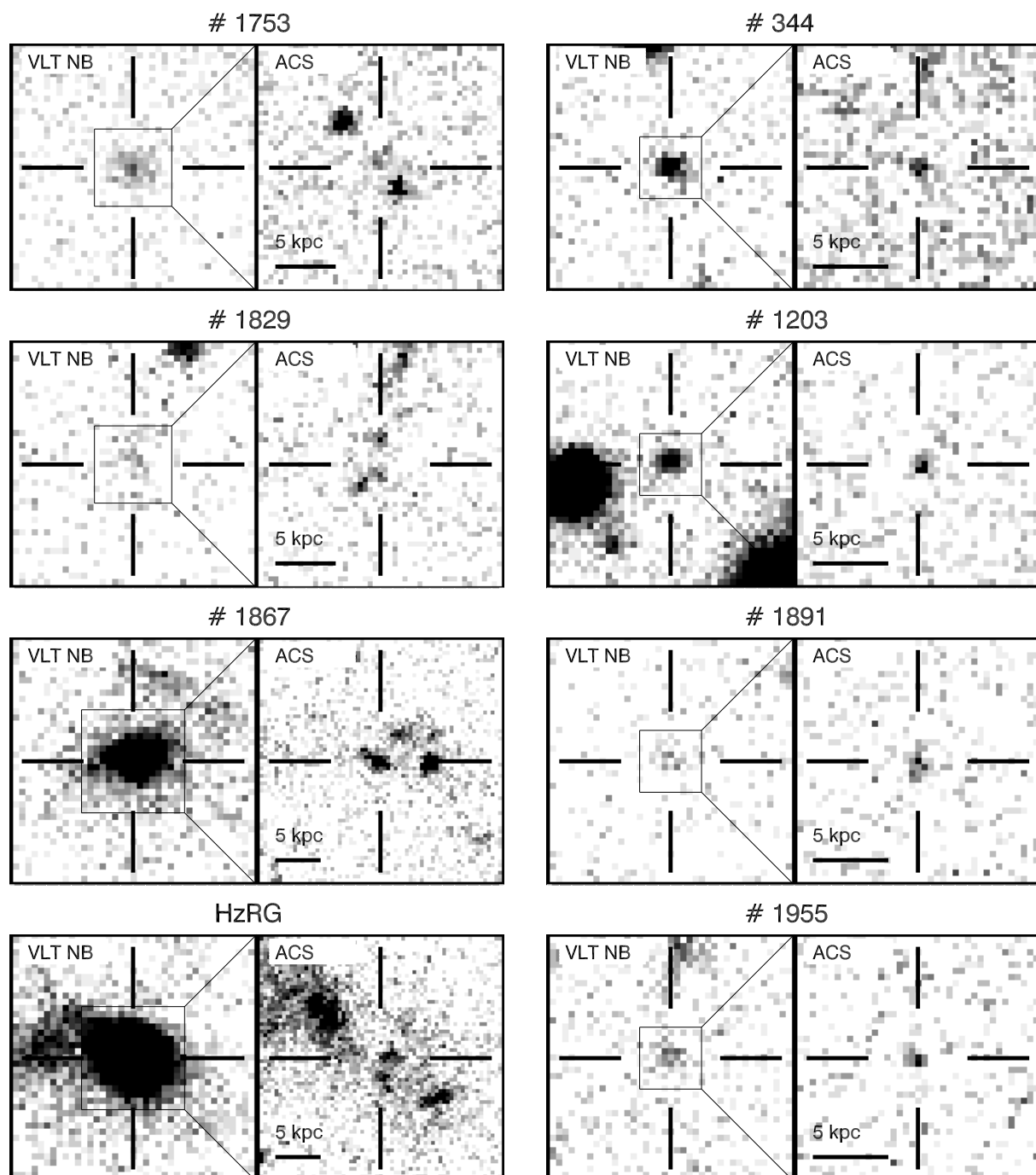
Figure 3.14 — VLT narrow-band and ACS images of \text{Ly}\alpha emitters with a clumpy counterpart ( left ) and of emitters that remained unresolved in the ACS image ( right ). The cutouts of the narrow-band image are \sim 8'' on the side. The ACS images are zoomed in on the centre of the narrow-band image. The grayscale ranges from 0.5 to 5 times the rms background noise. The emission to the left of the radio galaxy in the VLT image (and in the top-left corner of the ACS image) are from a foreground galaxy at z \sim 0.87 (see also §3.6).
