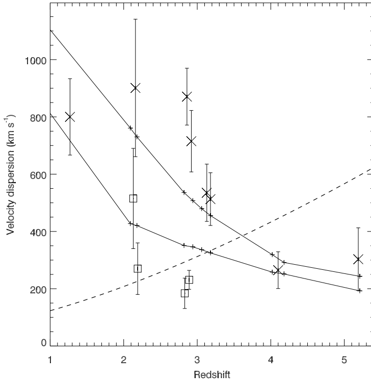
Figure 7.4 — Velocity dispersion of \text{Ly}\alpha emitters in the radio galaxy protoclusters ( crosses ). The squares represent the velocity dispersion of the subgroups in the 1138 and 0052 fields (see Chapter 5 for the details). The data point near z = 1.24 represents the velocity dispersion in the X-ray cluster RDCS 1252.9-2927. The solid lines show the evolution of the velocity dispersion of the galaxies in two of the simulated clusters. The dashed line shows the Hubble flow over 1 Mpc as a function of redshift.
