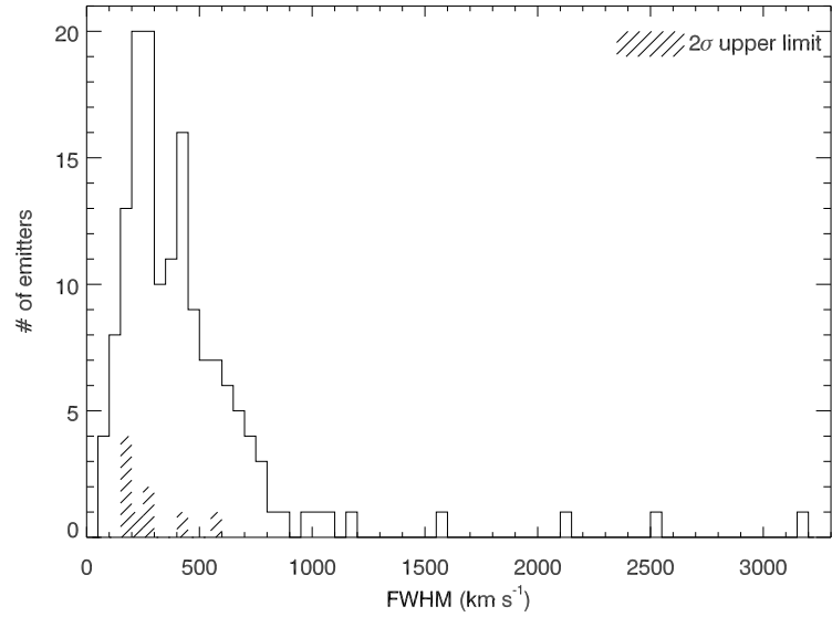
Figure 6.1 — Distribution of the FWHM of 153 confirmed galaxies with a \text{Ly}\alpha emission line. For lines that remained unresolved, 2\sigma upper limits are given.
