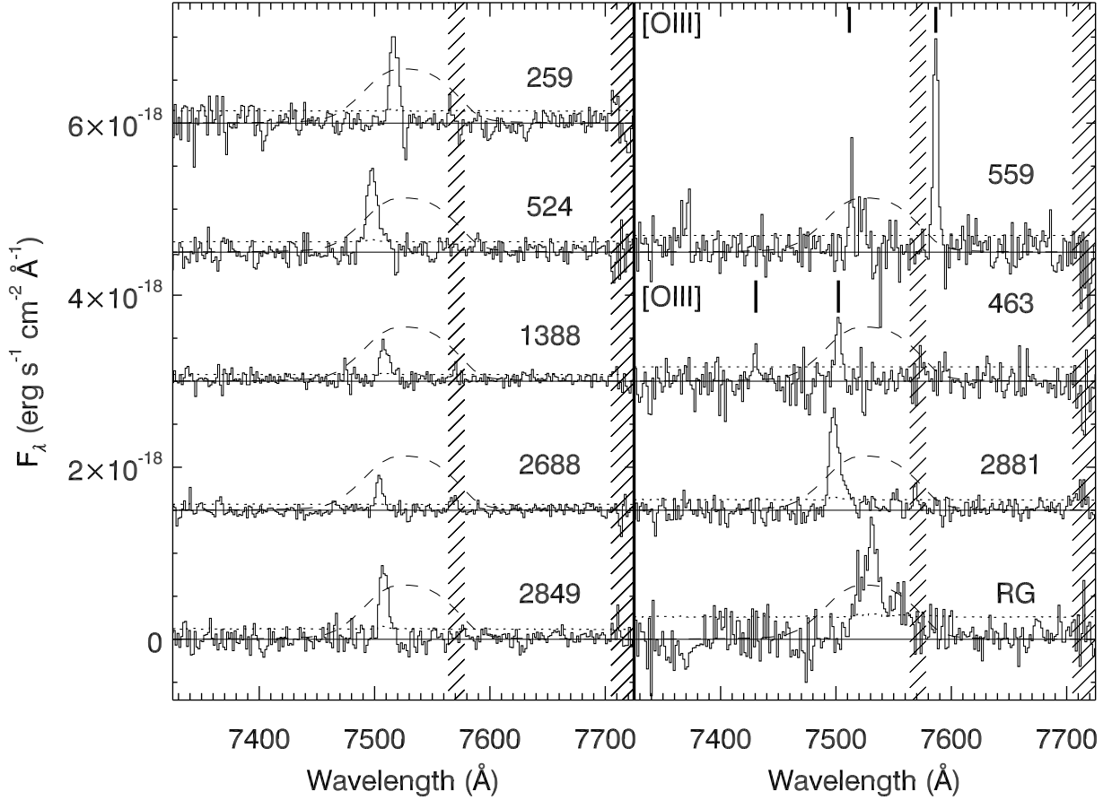
Figure 4.1 — Part of the spectra of the eight spectroscopically observed high priority emitters and the radio galaxy. For clarity the spectra are offset by 1.5 \times 10^{-18} \text{ erg s}^{-1} \text{ cm}^{-2} . The solid lines indicate the zero point of the spectra, the dotted lines the 1\sigma uncertainty in the data, and the dashed lines are the scaled transmission curves of the narrow-band filter. The regions in the spectrum where strong telluric skylines dominate are indicated with hashed lines.
