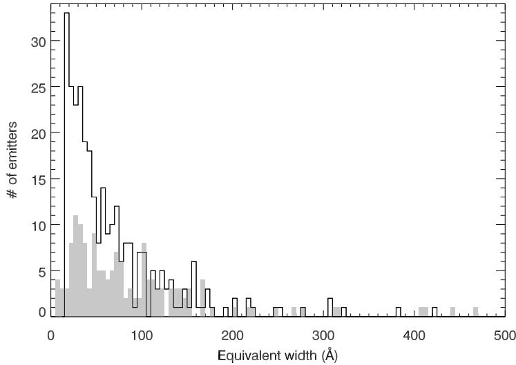
Figure 6.8 — The distribution of rest-frame equivalent width of 298 candidate \text{Ly}\alpha emitters in eight high redshift radio galaxy fields. The solid grey histogram represents the equivalent width distribution of the 153 confirmed \text{Ly}\alpha emitters in these fields.
