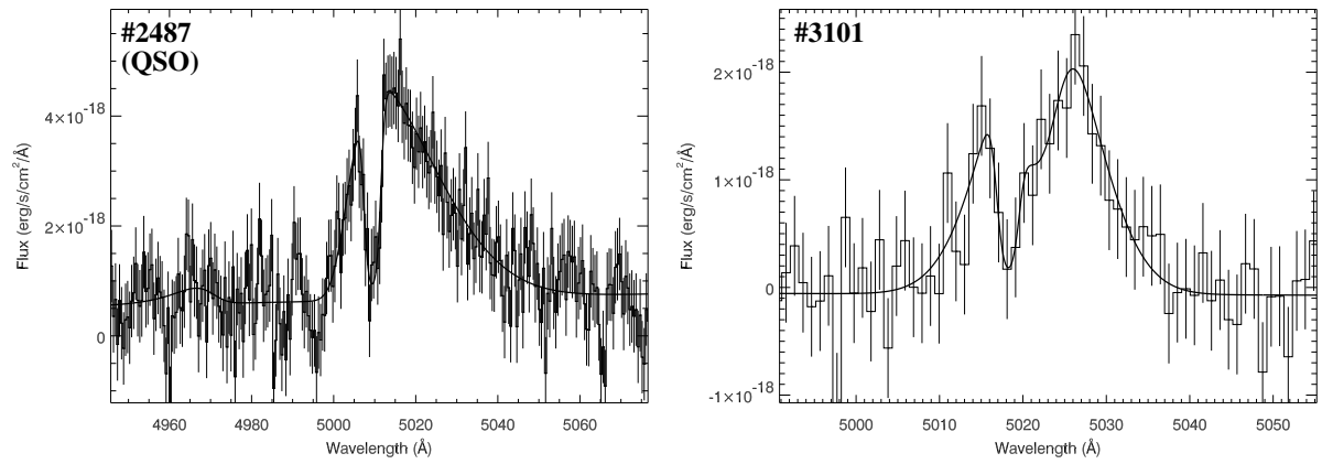
Figure 3.10 — Spectra of emitter #2487 (left) and #3101 (right).
