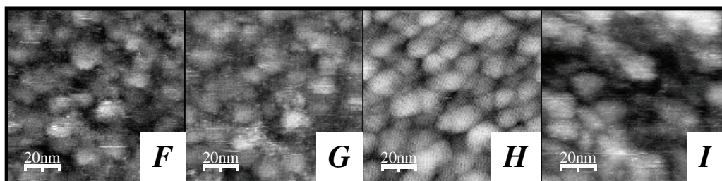
Figure A.II.6: STM images ( 100\text{nm}\times 100\text{nm} ) reflecting the morphology of the Pt (111) surface while exposed to 1.25 bar of C_2H_2 (images F and I) or/and 1.25 bar of O_2 (images G and H). V_t=0.1 V, I_t=0.2 nA.
