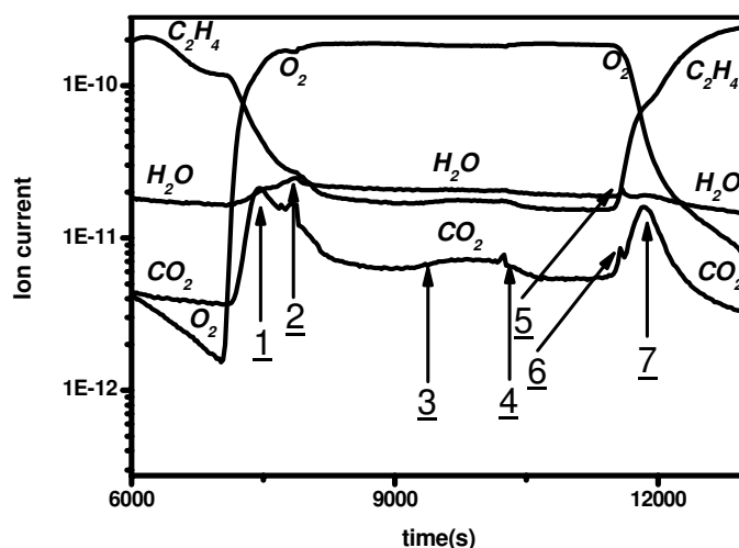
Figure A.II.5: Reaction kinetics for the total oxidation of ethene on Pt (111) as recorded by the quadrupole mass spectrometer. P_{total} = 1.25 bar, T = 413 K.
