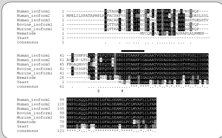
Figure 1 Alignment of the human, bovine, murine, C. elegans , and yeast Subunit c protein sequences. The sequence alignment of unprocessed predicted Subunit c protein of the mitochondrial ATP synthase shows strong conservation in the carboxy-terminal half of the protein. Conserved amino acids are depicted in black boxes, neutral substitutions in grey boxes. The consensus sequence is indicated by asterisks when completely conserved and by dots when more than 50% conserved between species. The cleavage site predicted to be used during the processing of the C. elegans preprotein (§), the first eleven amino acid peptide of the mature Subunit c protein used by Kominami [33] to raise antibodies (bar), and the amino acid before which the GFP sequence was inserted to create the GFP-Subunit c fusion protein (#) are indicated.
