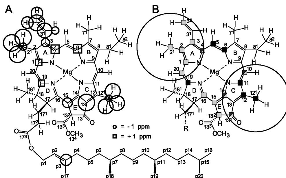
Fig. 1.3. (A) Visual representation of the carbon and proton aggregation shifts ( \Delta\sigma ) for aggregated Chl a. The circles around the carbon and hydrogen atoms represent upfield aggregation shifts, squares represent downfield shifts. The sizes of the circles and squares reflect the magnitude of the aggregation shifts. (B) Schematic representation of the assignment of heteronuclear correlations involving the 2^1\text{-H}_3 , which are shown in shaded grey or the 12^1\text{-H}_3 , which are solid black. For the 4-C, 10-C, 13^1\text{-C} and 14-C the correlations with proton signals are assigned to transfer from both methyl groups. The ranges for intramolecular transfer for the two methyl groups are indicated with the circles. Intramolecular correlations involving the 3^1\text{-C} and 13-C could not be assigned. Reprinted from ref. [19].
