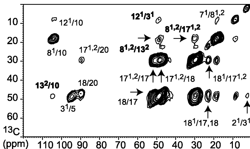
Fig. 4.3. ^{13}\text{C} - ^{13}\text{C} \text{CP}^3 spectrum recorded in a field of 9.4 T using a mixing time of 200 \mu\text{s} . The intermolecular correlations are indicated in bold type.
