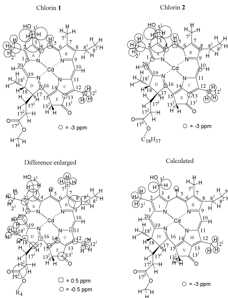
Fig. 5.8. Detected ^1\text{H} and ^{13}\text{C} aggregation shifts of aggregated chlorin 1 and 2 relative to the monomers in DMSO- d 6 , the enlarged difference between the aggregates (chlorin 2 minus chlorin 1 ) and calculated ^1\text{H} ring current shifts > 2.5 ppm. The circles have a radius proportional to the magnitude of the shift.
