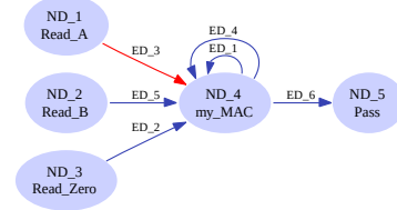
Figure 8.4: Matrix Multiplication: only FIFO implementation version
