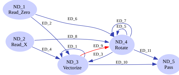
Figure 8.6: The QR Process Network
