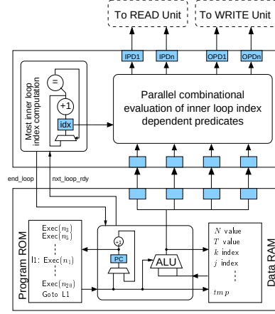
Figure 3.6: Partitioned hardware loop controller architecture
