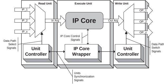
Figure 2.4: The Virtual Processor synthesis template
