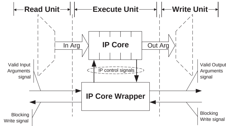
Figure 7.2: The Execute unit template
