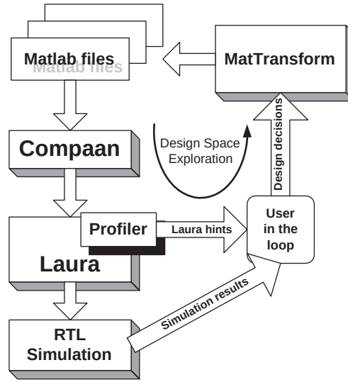
Figure 7.7: The modified COMPAAN/LAURA tool chain with feedback
