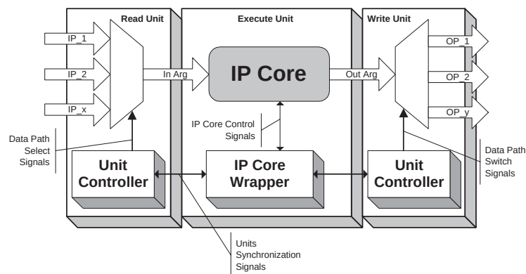
Figure 3.1: The Virtual Processor template
