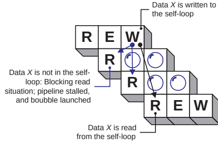
Figure 7.8: Data Hazard in Virtual Processor template
