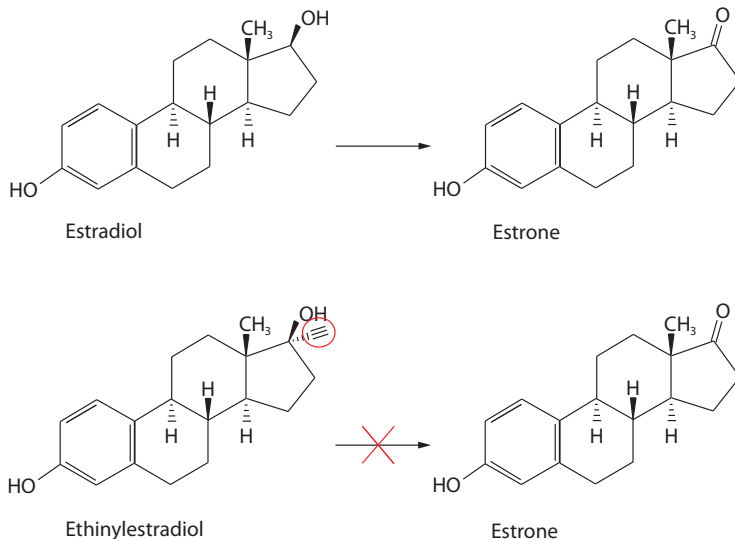
Figure 1.1: The oxidation at C-17 of estradiol to estrone is shown in the top part. This oxidation is blocked by the ethinyl-group in ethinylestradiol (indicated by circle) depicted in the bottom part
