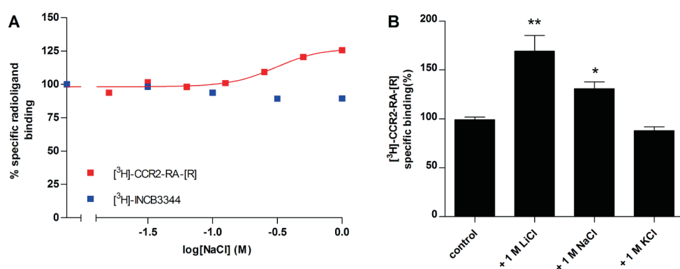
Fig. 3. (A) Modulation of binding of the orthosteric antagonist [ ^3\text{H} ]-INCB3344 and the allosteric antagonist [ ^3\text{H} ]-CCR2-RA-[R] to CHO cell membranes transiently expressing CCR2 by increasing concentrations of NaCl. Results are presented as percentage of bound radioligand for one representative experiment performed in duplicate. (B) Modulation of binding of the allosteric antagonist [ ^3\text{H} ]-CCR2-RA-[R] by 1 M LiCl, NaCl or KCl. Results are presented as mean \pm S.E.M. for at least three independent experiments performed in triplicate. * p < 0.05 vs. control, ** p < 0.005 vs. control, Student's t -test.
