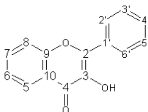
Figure 6.1. A representation of the flavonol skeleton. The flavonol ring and atom nomenclature is given in the Figure. Quercetin is obtained by inserting hydroxy (OH) substituents at positions 5, 7, 3' and 4'. Alternative 2,3 QD substrates are kaempferol where OH substituents are present at 5,7 and 4', galangin (OH at 5 and 7), fisetin (OH at 7, 3' and 4') and myricetin (OH at 5,7,3',4' and 5'). Compared to quercetin the relative degradation rate for the different substrates by Aspergillus flavus is 2.54, 0.30, 0.58 and 0.87 respectively (Oka et al. , 1972).
