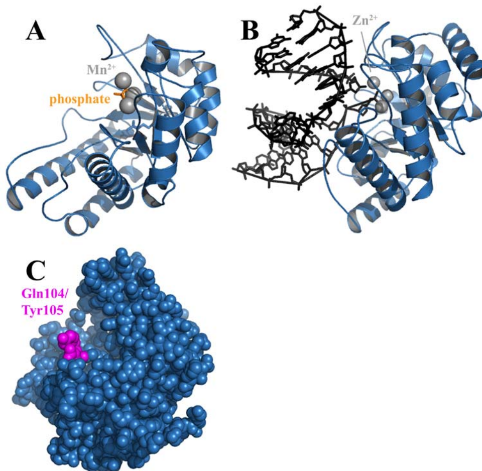
Fig. 10 Crystal structures of UVDE and Endonuclease IV. (A) UVDE containing three Mn^{2+} metal ions (gray spheres) and a phosphate molecule (orange) (pdb accession number 2J6V). (B) Endonuclease IV bound to dsDNA containing tetrahydrofuran as a synthetic abasic site (pdb accession number 1QUM). The substrate exhibits a nick directly 5' to the lesion due to cleavage by the protein. The structure shows three Zn^{2+} metal ions (gray). The DNA is shown in black. (C) Different view of the UVDE protein showing the DNA-binding groove and the two residues Gln104 and Tyr105 in magenta. Proteins are indicated in blue.
