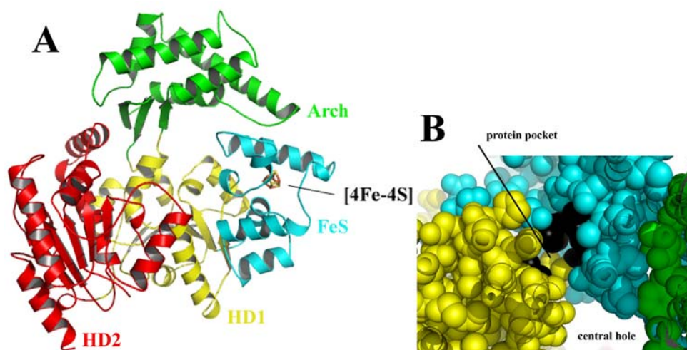
Fig. 20 Crystal structure of the Thermoplasma acidophilum XPD protein (pdb accession number 2VSF). (A) Full structure. The two helicase domains (HD1-2, yellow and red), the FeS domain (cyan) and the Arch domain (green) are indicated. The 4Fe-4S cluster is also shown. (B) Close-up view of the pocket present in the crystal structure. Residues forming the pocket (Arg88, Tyr166 and Tyr185) are shown in black.
