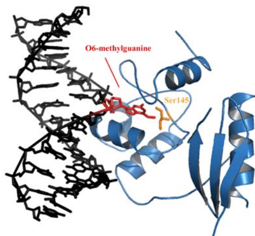
Fig. 1 Crystal structure of the human alkylguanine-DNA alkyltransferase (AGT) bound to dsDNA containing an O 6 -methylguanine adduct (pdb accession number 1T38). The protein is indicated in blue and the DNA in black. The extrahelical nucleotide is highlighted in red and is in close vicinity to the catalytic cysteine, which in the protein used for the co-crystal has been replaced by serine (orange).
