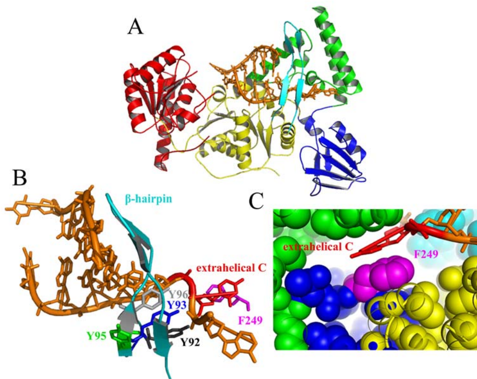
Fig. 15 Crystal structure of the UvrB protein bound to a small DNA loop (pdb accession number 2FDC). (A) Crystal structure of the UvrB protein bound to DNA. Colors are identical to figure 14 and denote the domain organization of UvrB. DNA is indicated in orange. (B) Zoom-in representation of the structure showing the \beta -hairpin (cyan) and residues Tyr92 (black), Tyr93 (blue), Tyr95 (green), Tyr96 (gray) and Tyr249 (magenta). The extrahelical cytosine is indicated in red. (C) Space-filling representation showing the planar pocket of the UvrB protein. The extrahelical cytosine (red) undergoes a stacking interaction with Tyr249 (magenta).
