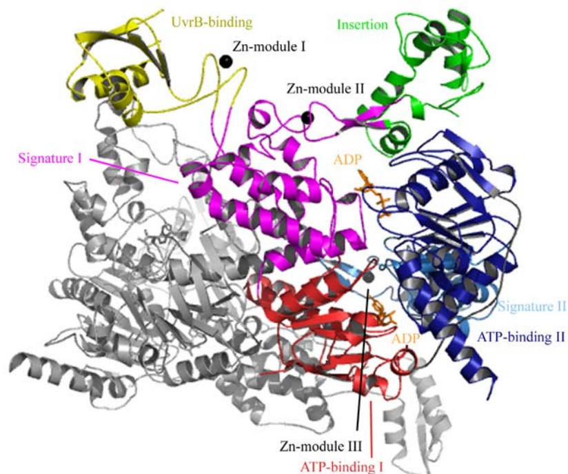
Fig. 12 Crystal structure of the UvrA dimer from B. stearothermophilus (pdb accession number 2R6F ). In the structure the different domains of UvrA are indicated. NBD-I consists of ATP-binding domain I and Signature domain I, whereas NBD-II consists of ATP-binding domain II and Signature domain II. Zn-ions are shown as black spheres and the ADP molecules in orange. The second UvrA monomer is indicated in grey.
