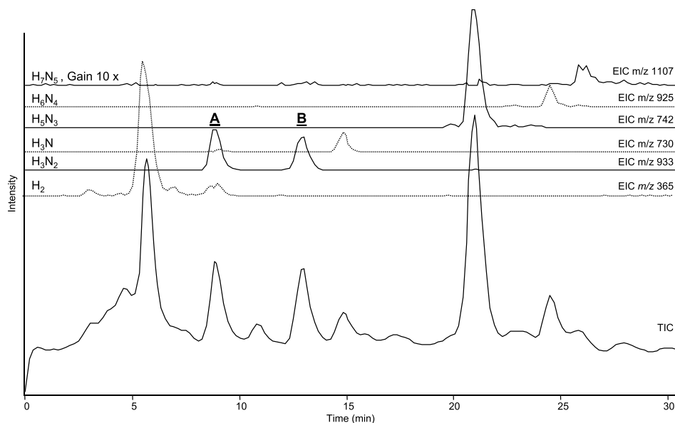
Figure 3-6. HPAEC-on-line-MS of oligosaccharides from the urine sample of a G_{M1} -gangliosidosis patient. TIC is the total ion chromatogram. The extracted ion chromatograms (EIC) represent the major pseudomolecular ions registered. Several of the EIC show the separation of isobaric structures. Fragmentation analysis of the well-separated H_3N_2 species A and B is shown in Fig. 3-7. H, Hexose; N, N -acetylhexosamine.
