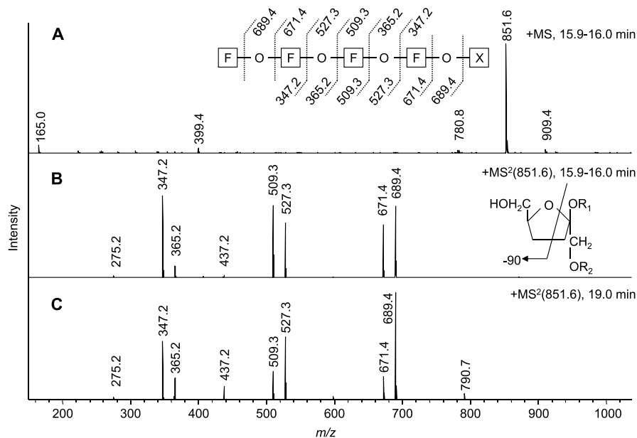
Figure 3-4. Mass spectra of the two isobaric sodium adducts of DP5 fructans. Part (A) shows the MS spectrum of [GF_4 + Na]^+ ; parts (B) and (C) are the MS^2 spectra with m/z 851.6 as precursor ion, where (B) represents GF_4 and (C) F_5 . In the fragmentation scheme, F stands for fructofuranosyl and X is glucopyranosyl or fructopyranosyl, R_1 and R_2 stand for the rest part of the oligosaccharide chain and R_2 can also be a H.
