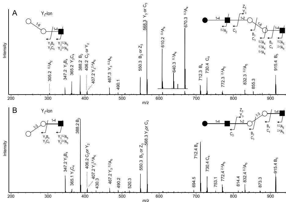
Figure 3-7. Fragment ion analysis of H 3 N 2 species. H 3 N 2 species A and B, as indicated in Fig. 3-6, were subjected to MS 2 analysis in their sodiated form ( m/z 933.5; A and B, respectively). The observed fragment ions are schematically interpreted according to the nomenclature of Domon and Costello [26]. Empty circle, mannose; filled circle, galactose; filled square, N -acetylglucosamine.
