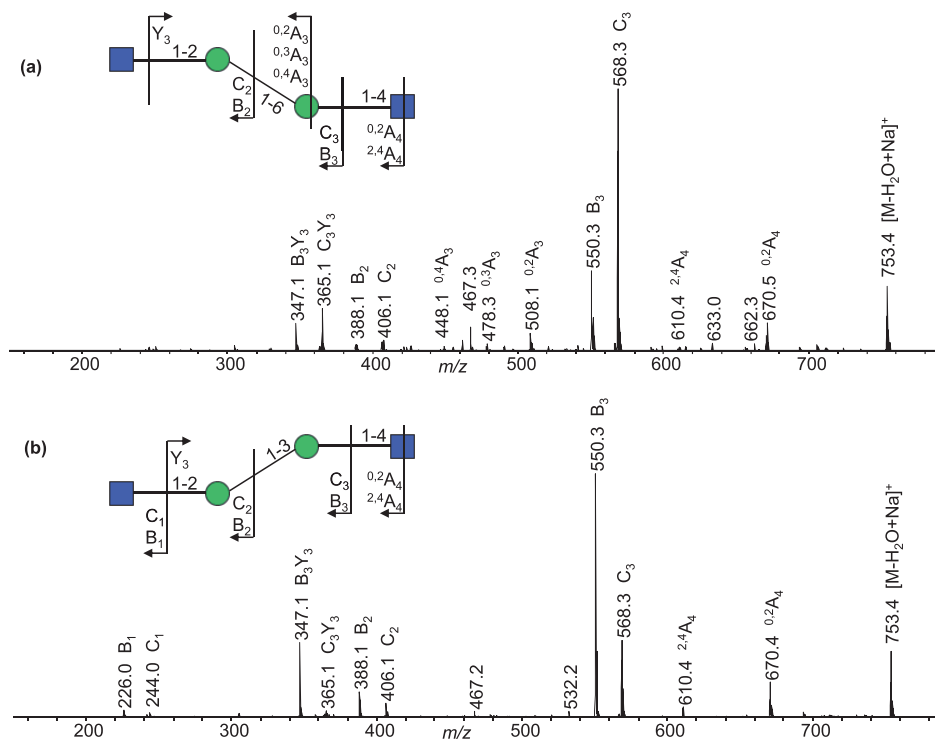
Figure 5-8. Positive-ion fragmentation mass spectra of two isomeric monosodiated tetrasaccharides \text{Hex}_2\text{HexNAc}_2 (precursor ion at m/z 771.5) from urine of a \text{G}_{\text{M}2} -gangliosidosis patient. The separation of A and B is shown in Fig. 5-7. Green circle = mannose, blue square = N-acetylglucosamine.
