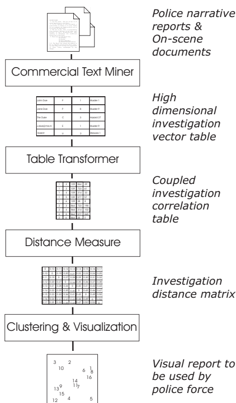
Figure 9.1: Four-step paradigm
