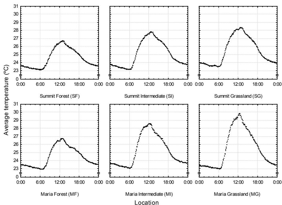
Figure 3: Daily temperature curves for the six habitats during the first field experiment period. The measurements were made between August 21 st and September 23 rd 1998, with time interval of 6 minutes, and temperatures are averaged per measurement per interval over 33 days. The left two graphs are for the forest locations, the middle two graphs for the intermediate locations and the right two graphs for the grassland populations.
