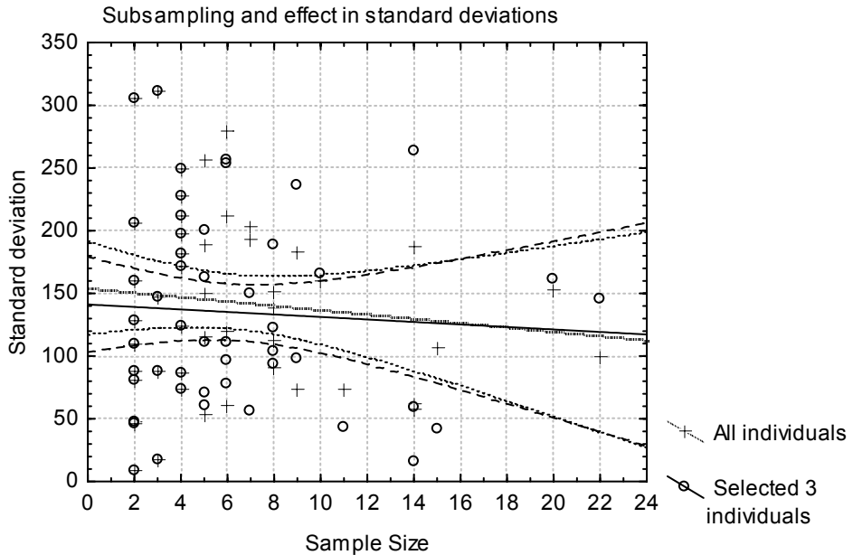
Figure 2: Impact of sub-sampling on the estimated standard deviations for dry weight. Sub-samples were obtained from around the median of the family samples of the D. malerkotliana dataset.
