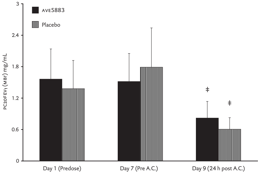
FIGURE 3 Airway responsiveness to mbr expressed as PC 20 FEV 1 (mBR) on days 1,7 and 9 during both AVE5883 (filled bars) and P (striped bars) treatment period. Allergen challenge decreased PC 20 FEV 1 (mBR) during both treatment periods (day 7 vs. 9), ‡ = P<0.05. However, there was no significant difference in the changes in allergen-induced airway responsiveness to MBR between the two treatments (p=0.21).
