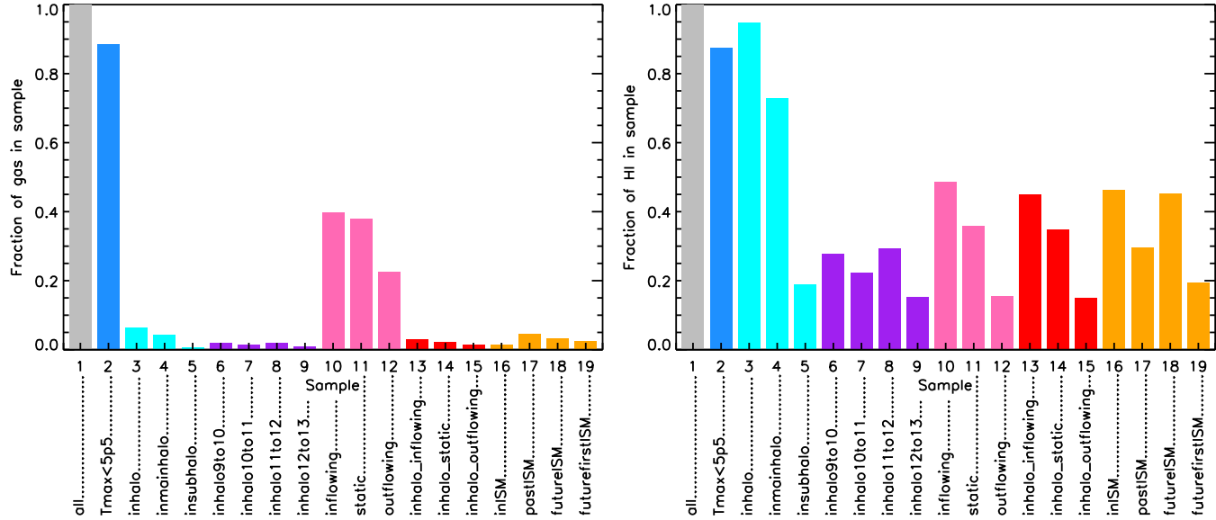
Figure 5.1: Fraction of the total amount of gas (left) and H\text{I} (right) at z = 3 accounted for by the selections listed in Table 5.1. Many samples (#3–9 and #13–19) contain a much larger fraction of the H\text{I} mass than of the total gas mass.
