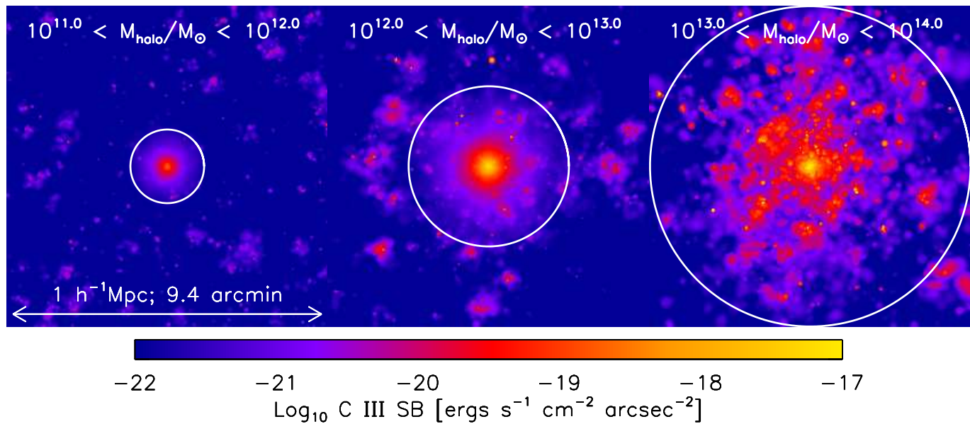
Figure 6.4: Mean C III emission maps for haloes with M_{\text{halo}} = 10^{11-12} M_{\odot} , M_{\text{halo}} = 10^{12-13} M_{\odot} , and M_{\text{halo}} = 10^{13-14} M_{\odot} , from left to right, at z = 0.125 . The images are 1 h^{-1} comoving Mpc on a side, span 9.4 arcmin on the sky, and have a pixel size of 2 arcsec. The white circles indicate the median virial radius.
