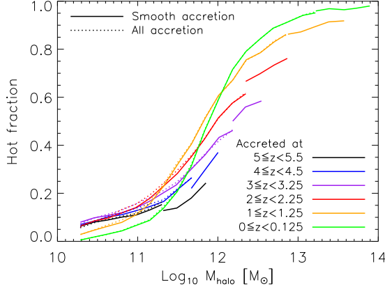
Figure 2.11: Hot fraction for accretion onto haloes just before z = 5, 4, 3, 2, 1 , and 0 against halo mass at the same redshift. The curves at low halo masses are obtained from simulation REF_L050N512 . At the high-mass end we have added curves for simulation REF_L100N512 to extend the dynamic range. Gas is considered to have been accreted hot if it has T_{\text{max}} \geq 10^{5.5} . The dotted curves show the hot fraction including both smooth accretion and mergers. Each mass bin contains at least 10 haloes. For a fixed halo mass, hot accretion tends to be more important at lower redshift.
