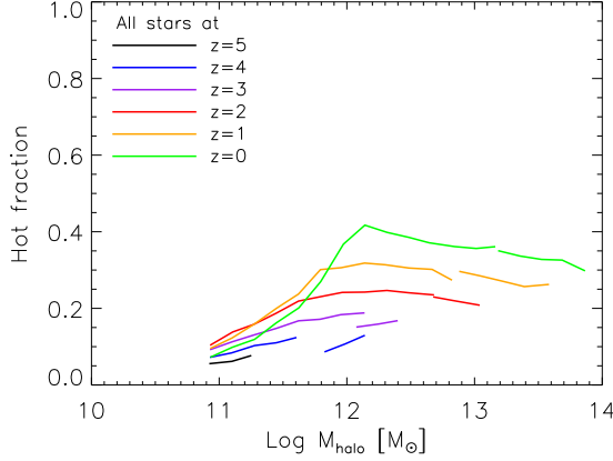
Figure 2.18: Fraction of the stellar mass at the indicated redshifts, that formed from gas that had earlier reached temperatures exceeding T_{\text{max}} \geq 10^{5.5} K, as a function of the host halo mass at the corresponding redshifts for the simulation REF_L050N512 . We added the highest mass bins from REF_L100N512 to extend the dynamic range. Each mass bin contains at least 10 haloes. At any time and for any halo mass, hot mode accretion contributed less than 40% to the total stellar mass.
