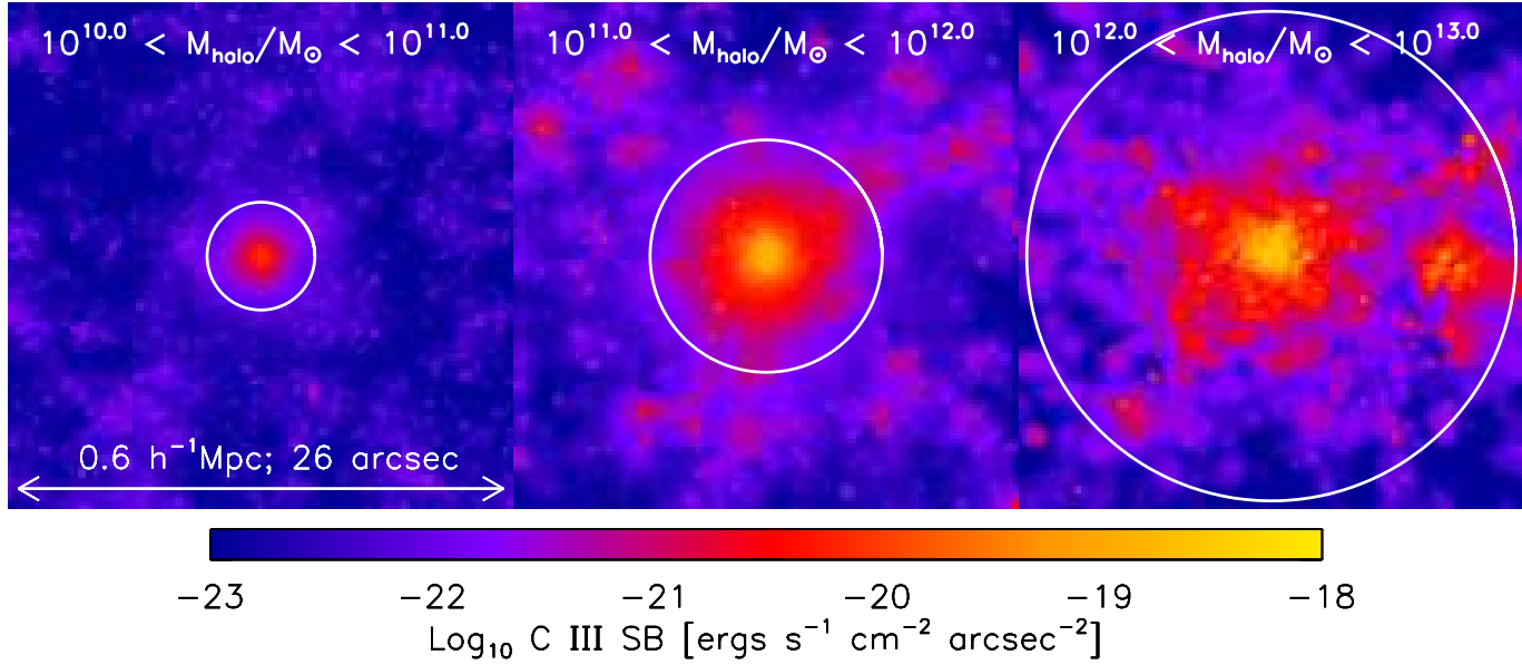
Figure 6.7: Mean C III emission maps for haloes with M_{\text{halo}} = 10^{10-11} M_{\odot} , 10^{11-12} M_{\odot} , and 10^{12-13} M_{\odot} , from left to right, at z = 3 . The images are 0.6 h^{-1} comoving Mpc on a side, span 26 arcsec on the sky, and have a pixel size of 0.2 arcsec. The white circles indicate the median virial radius.
