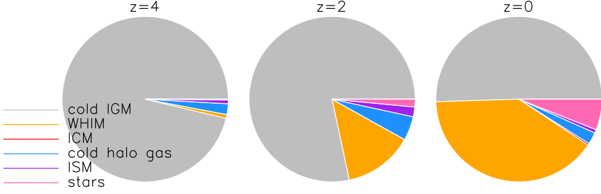
Figure 1.2: Distribution of baryonic matter amongst the different gas phases and stars. The cold IGM (grey) dominates, but becomes less important towards lower redshift. The WHIM (orange) becomes more important towards lower redshift. The ICM (red) is never very important. The amount of cold halo gas (blue) and ISM (purple) is largest at z \approx 2 . The stellar mass keeps building up down to z = 0 . The simulation used is the reference simulation in a (50 h^{-1} \text{Mpc})^3 volume from the OWLS project (Schaye et al., 2010).
