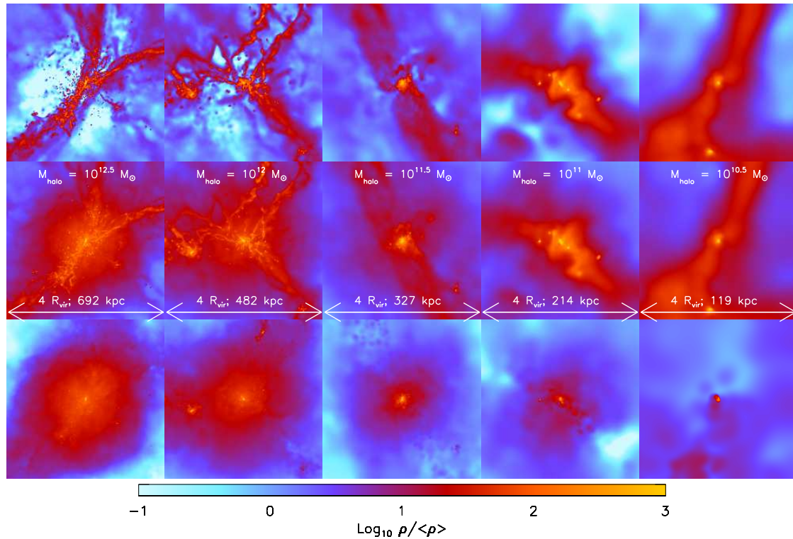
Figure 4.1: Gas overdensity at z=2 in and around haloes with, from left to right, M_{\text{halo}} = 10^{12.5}, 10^{12}, 10^{11.5}, 10^{11}, and 10^{10.5} M_{\odot} taken from the simulation REF_L025N512 . All images show projections of the gas density in cubes of 4 virial radii on a side. The proper sizes of the images are indicated in the panels of the middle row. In the middle column all gas was included. In the top (bottom) row we have only included cold- (hot-) mode gas, i.e. gas with T_{\text{max}} < 10^{5.5} \text{ K} ( T_{\text{max}} \geq 10^{5.5} \text{ K} ). The filaments, streams, and dense clumps consist of gas that has never been heated to temperatures greater than 10^{5.5} \text{ K} .
