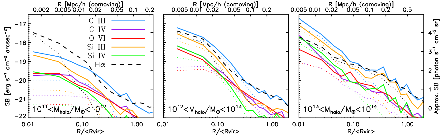
Figure 6.5: Mean UV (solid curves) and H \alpha (dashed curve) surface brightness as a function of radius at z = 0.125 for the same haloes as in Figure 6.4. The emission lines are indicated in the legend. Dotted curves show the median profile. The radius is normalized by dividing by the median virial radius in each mass bin. The surface brightness in \text{erg s}^{-1} \text{cm}^{-2} \text{arcsec}^{-2} on the left y-axis is exact. It has been converted to \text{photon s}^{-1} \text{cm}^{-2} \text{sr}^{-1} using \langle \lambda \rangle = 1232 \text{ \AA} . The pixel size was 2 arcsec before it was binned and the thickness of the region is 2.2 h^{-1} comoving Mpc. C III is the brightest line, followed by Si III.
