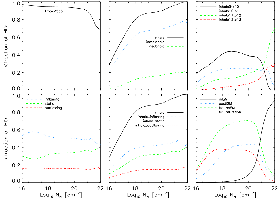
Figure 5.4: Mean fraction of the H I column density at z = 3 contributed by the gas which fulfils the selection criteria listed in Table 5.1 as a function of the total H I column density. Almost all of the contributing gas has T_{\text{max}} < 10^{5.5} K although hot-mode gas becomes significant, accounting for up to 30 per cent of the absorption, above 10^{21} \text{ cm}^{-2} . More than 80 per cent of N_{\text{HI}} > 10^{18} \text{ cm}^{-2} gas is located inside (main) haloes. About 55 per cent of the H I is inflowing, but the contributions from static and outflowing gas are about 30 and 15 per cent, respectively, and therefore not negligible. The contribution from gas accreting onto galaxies, i.e. gas that will join the ISM in the near future, is dominant for 10^{17} - 10^{21} \text{ cm}^{-2} , accounting for up to 70 per cent. Strong DLAs ( N_{\text{HI}} > 10^{21} \text{ cm}^{-2} ) are dominated by ISM gas (contributing more than 60 per cent to the absorption) and the Lyman- \alpha forest by gas that will remain intergalactic down to at least z = 2 (contributing more than 60 per cent to the absorption).
