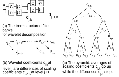
Figure 5.2: Wavelet decomposition.
