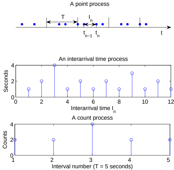
Figure 2.1: An example of a point process and its two representations: an interarrival time process and a count process.
