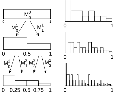
Figure 5.1: Binomial cascading process.
