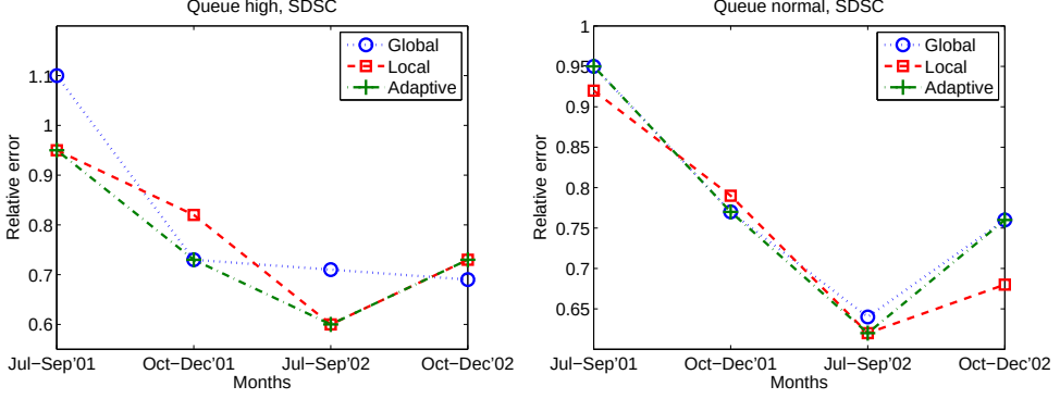
Figure 8.7: Relative generalization errors of global, local, and adaptive tuning for two representative queues on the SDSC trace. Adaptive tuning provides a lower bound of prediction errors compared to global and local tuning. Nevertheless, adaptive tuning is considered “conservative” since in some cases it favors global tuning than local tuning even the latter achieves better accuracy.
