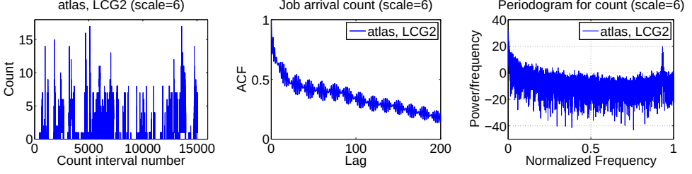
Figure 3.5: The sequence plot, autocorrelation function (ACF), and power spectrum via periodogram for the count process of atlas , LCG2 .
