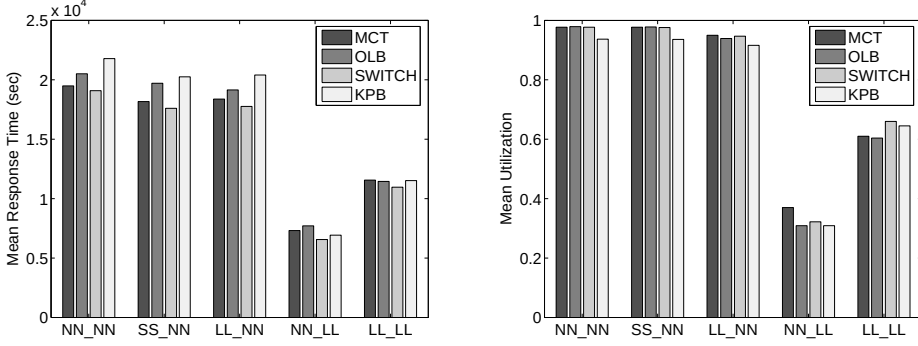
Figure 7.4: Performance comparison of four Grid scheduling heuristics. Workload structure is denoted as “Grid arrival” “Grid run time” “local arrival” “local run time”. N - Not dependent, S - Short range dependent, L - Long range dependent. For example, “NN_LL” means that the job arrival and run time series at the Grid level are not dependent, while the background workloads at the local level are long range dependent.
