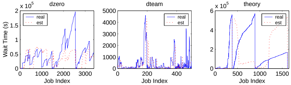
Figure 8.5: Comparisons of real and estimated queue wait times for three representative groups on the NIKHEF trace.
