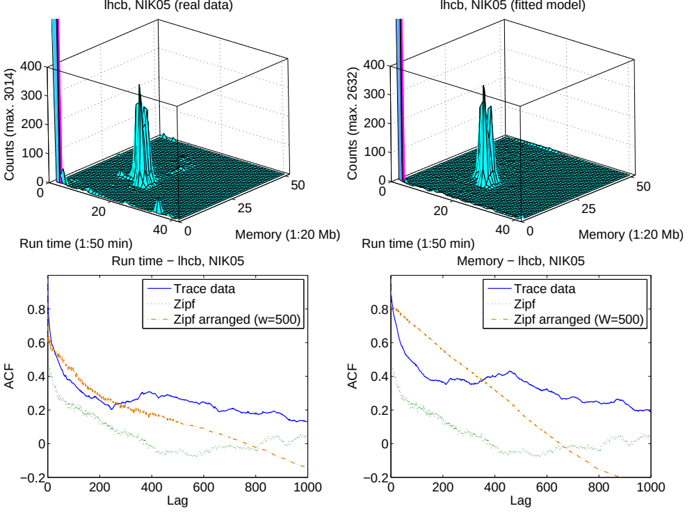
Figure 6.5: Fitting the joint distribution of run time and memory of lhcb , NIK05 ( G = 9 ). ACFs of these two attributes are plotted separately. The selected algorithms for synthetic data generation are the localized sampling algorithm without (Zipf) and with the cluster permutation procedure (Zipf arranged).
