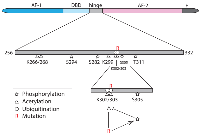
Figure 2: Posttranslational modifications in the ER \alpha hinge region. S305 phosphorylation prevents acetylation of K302/303. The natural K303R mutation blocks K302/303 acetylation and stimulates S305 phosphorylation.
