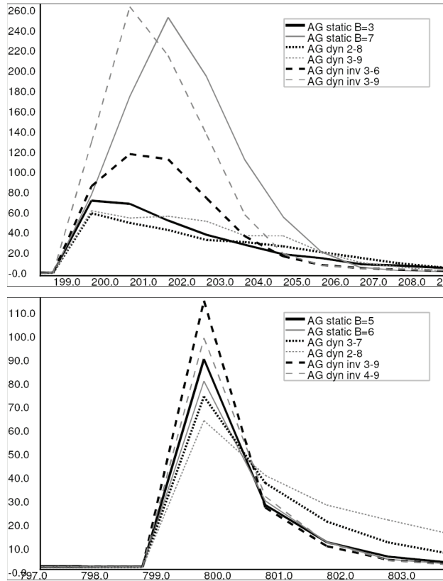
Figure 3.4. Alternating-Goal task; mean learning curves for phase 1 peak ( n=800 ). The mean number of steps (y-axis) needed to find the goal is plotted per trial for two static, two dynamic and two inverse-dynamic agents (see text for explanation).
