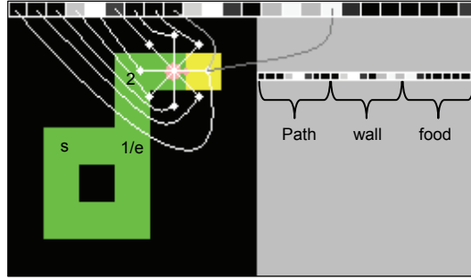
Figure 6.1. The experimental grid world. The agent is the “circle with nose” in the top right of the maze. In this figure the agent is looking to the right. The 8 white dots denote the points perceived by the agent. These points are connected to the elements of state s (neural input to the MLPs used by the agent) as depicted. This is repeated for all possible features, in our case: path (gray), wall (black), and
