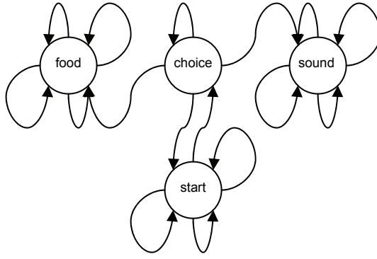
Figure 1.2 A state-transition diagram for the maze presented in Figure 1.1. Arrows denote move actions. Probabilities are assumed to be equal to 1 (i.e., choosing, for example, up always results in the state pointed to by the up-arrow). The states, sound and food are terminal states.
