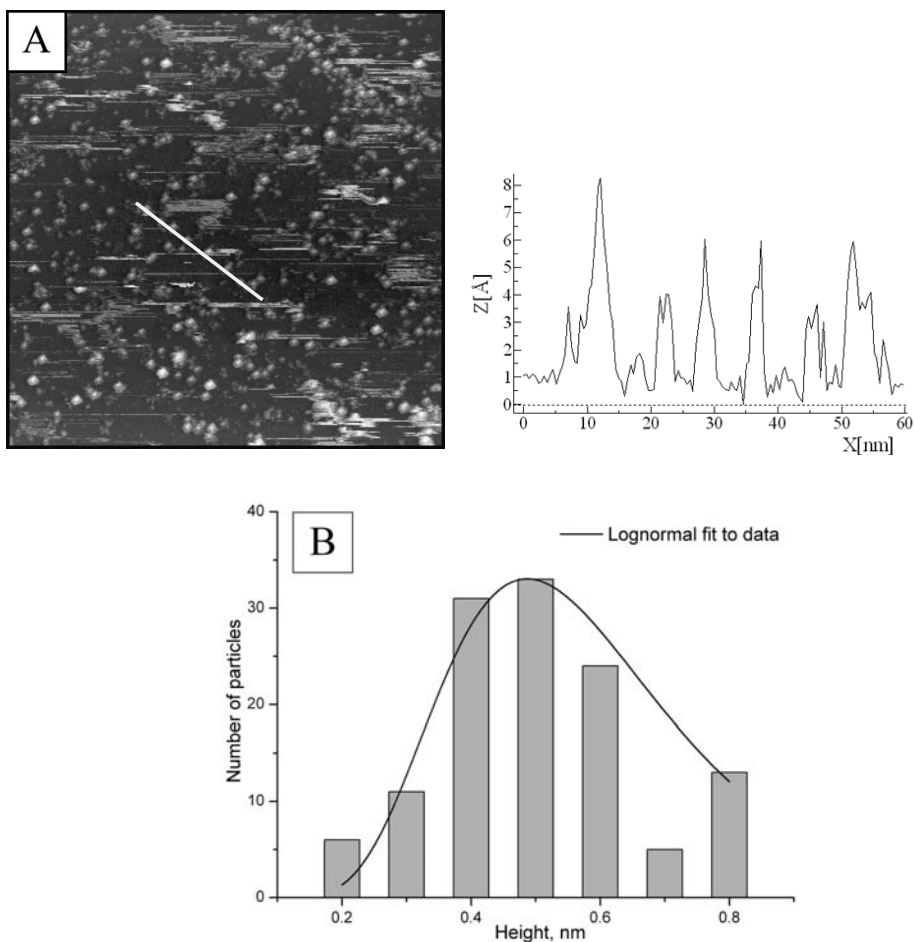
Figure 4.19: (A) STM- image ( 150 \times 150 \text{ nm}^2 ) of a Pt/HOPG sample with 0.2 ML Pt after annealing in \text{H}_2 for 1 h at 500^\circ\text{C} . (B) Height distribution histogram of Pt particles measured from multiple STM images taken in different sample locations. Particles within a range of heights \pm 0.03 \text{ nm} from the indicated values are grouped together.
