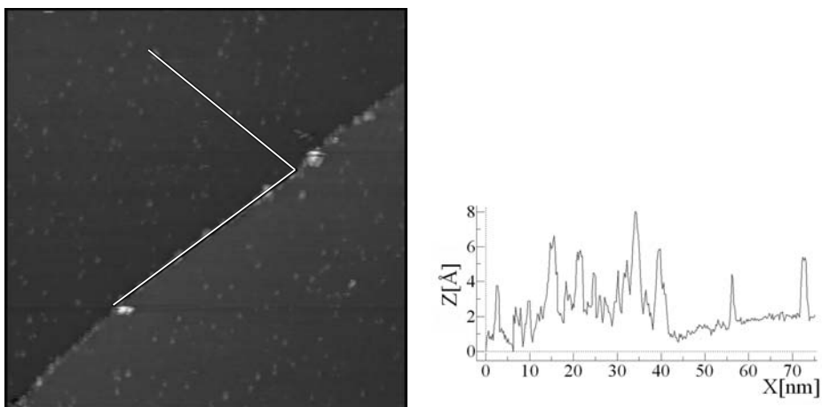
Figure 4.5: STM image ( 70 \times 70 \text{ nm}^2 ) of the HOPG(0001) surface with \sim 0.05 \text{ ML} of Pt and a line-profile along a step and a terrace. Imaging conditions: U_i = 0.2 \text{ V} , I_i = 0.1 \text{ nA} .
