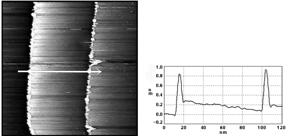
Figure 4.7: STM image ( 200 \times 200 nm 2 ) of HOPG with deposited \sim 0.05 ML Pt after annealing in UHV at 500 °C for 1.5 h showing two monoatomic steps decorated with Pt particles. Aside of the image, a line-profile, whose position is marked with the white line on the image, shows the apparent height of the particles situated near neighboring step edges. Imaging conditions: U_t = 0.2 V, I_t = 0.2 nA.
