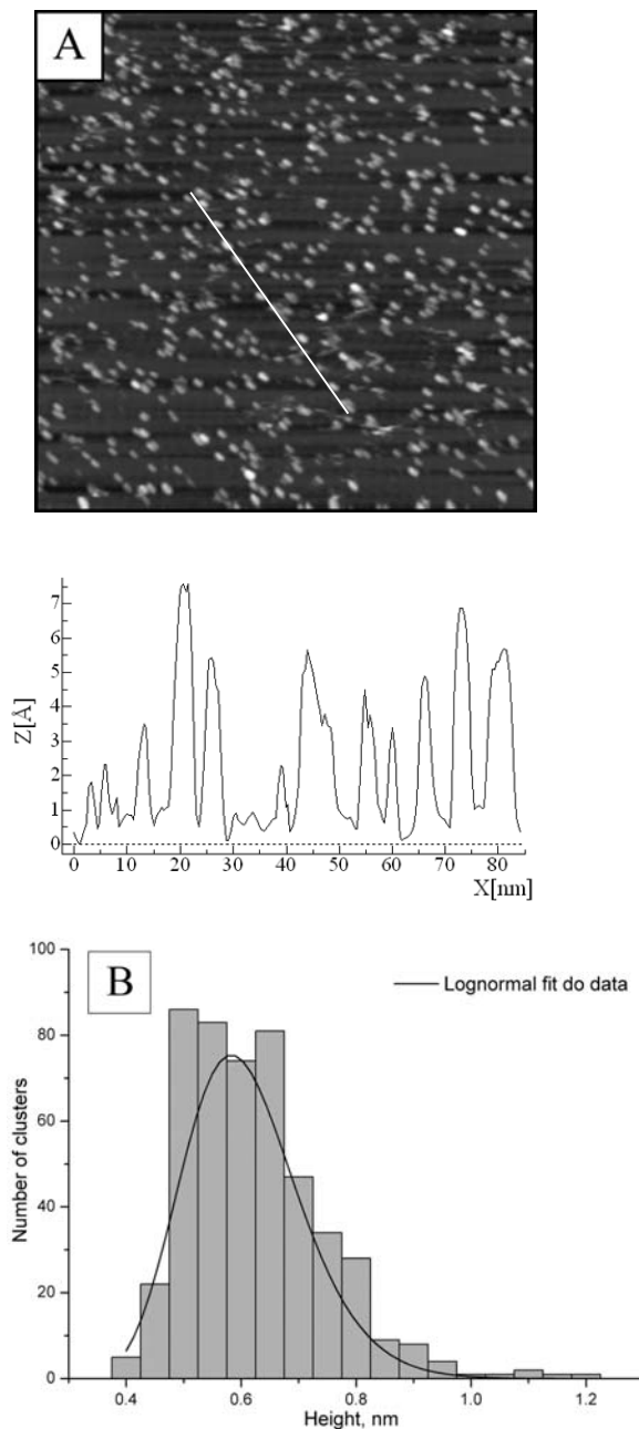
Figure 4.14: (A) STM-image ( 150 \times 150 \text{ nm}^2 ) of Pt/HOPG (0.2 ML Pt) after annealing in \text{O}_2 for 4 h at 500^\circ\text{C} . (B) Height distribution histogram of Pt particles on the same sample measured from multiple STM images taken in different sample locations. Particles within a range of heights \pm 0.03 \text{ nm} from the indicated values are grouped together.
