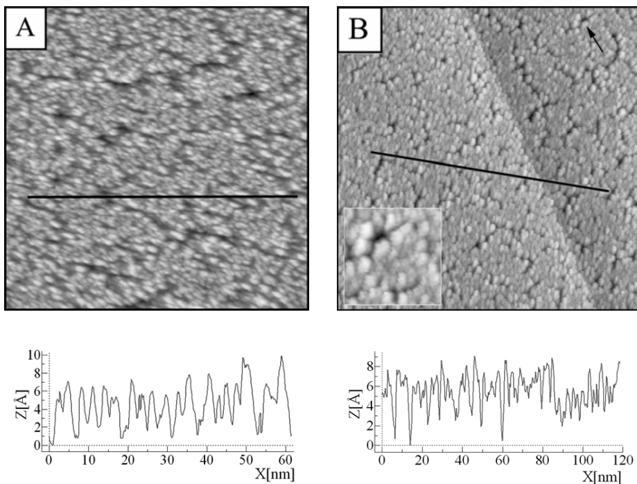
Figure 4.3: (A) STM image ( 70 \times 70 \text{ nm}^2 ) of 5 ML thick Pt film on HOPG and a line profile through the surface. (B) STM image ( 150 \times 150 \text{ nm}^2 ) of the same sample after annealing in UHV at 500^\circ\text{C} for 1 h and a line profile through the surface. The arrow on the image marks the location of the surface shown on the inset ( 20.1 \times 20.1 \text{ nm}^2 ). Imaging conditions: (A) U_t = 0.7 \text{ V} , I_t = 0.2 \text{ nA} , (B) U_t = -0.7 \text{ V} , I_t = 0.3 \text{ nA} .
