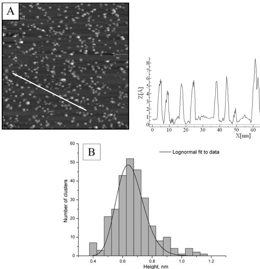
Figure 4.17: (A) STM-image ( 100 \times 100 \text{ nm}^2 ) of a Pt/HOPG sample with 0.4 ML Pt after annealing in CO for 3 h at 500^\circ\text{C} . (B) Height distribution histogram of Pt particles measured from multiple STM images taken in different sample locations. Particles within a range of heights \pm 0.03 \text{ nm} from the indicated values are grouped together.
