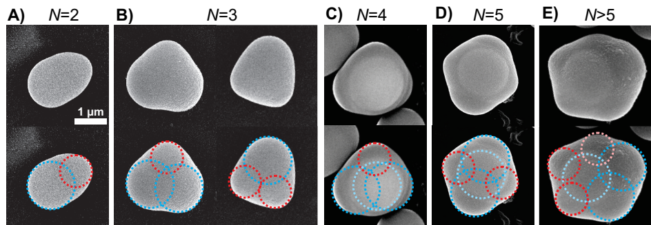
FIGURE 5.4: SEM micrographs of patchy particles constructed by 1.59 \mu\text{m} ( cd=1.6\% v/v ) and 1.06 \mu\text{m} ( cd=10\% v/v ) seed particles. Below the images a reconstruction of the spherical seed particles is shown. A) Asymmetric dumbbell constructed from one large and one small particle. B) The clusters of N=3 reconfigured to triangular shapes and consist of either two large and one small particle or one small and two large particles. C) Tetrahedron particle constructed by three large and one small sphere. D) Pentagonal dipyramid formed by three large and two small particles. E) Example of a cluster consisting of N>5 spheres. Reconstruction of the spherical seed particles indicates that the large spheres strongly deformed, whereas the smaller rigid particles maintained their spherical shape.
