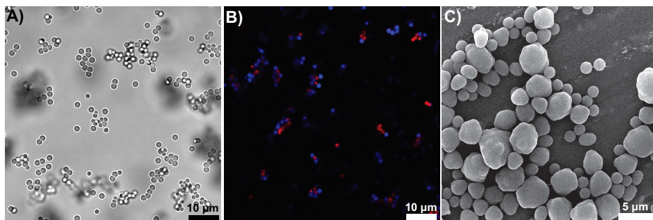
FIGURE 5.3: Applying the colloidal recycling method to a mixture of 1.06 \mu\text{m} polystyrene particles with cd = 10\% \text{ v/v} and 1.59 \mu\text{m} particles with cd = 1.6\% \text{ v/v} (size ratio of 1.5 and a crosslink density ratio of 6.3). A) Bright field microscopy image of randomly shaped aggregates after destabilization of the spheres. B) Confocal microscopy image of the aggregates with the 1.06 \mu\text{m} particles in red and the 1.6 \mu\text{m} seeds in blue. C) SEM micrograph of the reconfigured clusters obtained after reconfiguration and polymerization. Compact patchy shapes are formed of different sizes.
