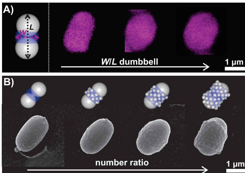
FIGURE 5.5: Dumbbell patchy particles consisting of two 1.06 \mu\text{m} spheres and various 0.23 \mu\text{m} spheres. A) Confocal microscopy images of dumbbell particles shaped from two 1.06 \mu\text{m} spheres with similar dumbbell lengths, but different dumbbell widths. B) SEM micrographs of dumbbells, where 0.23 \mu\text{m} spheres are positioned at the contact area between the large spheres. The width of the dumbbell increases with increasing number of 0.23 \mu\text{m} particles. At large number ratios the 0.23 \mu\text{m} particles arrange on an ordered lattice forming a 'jacket' around the dumbbell.
