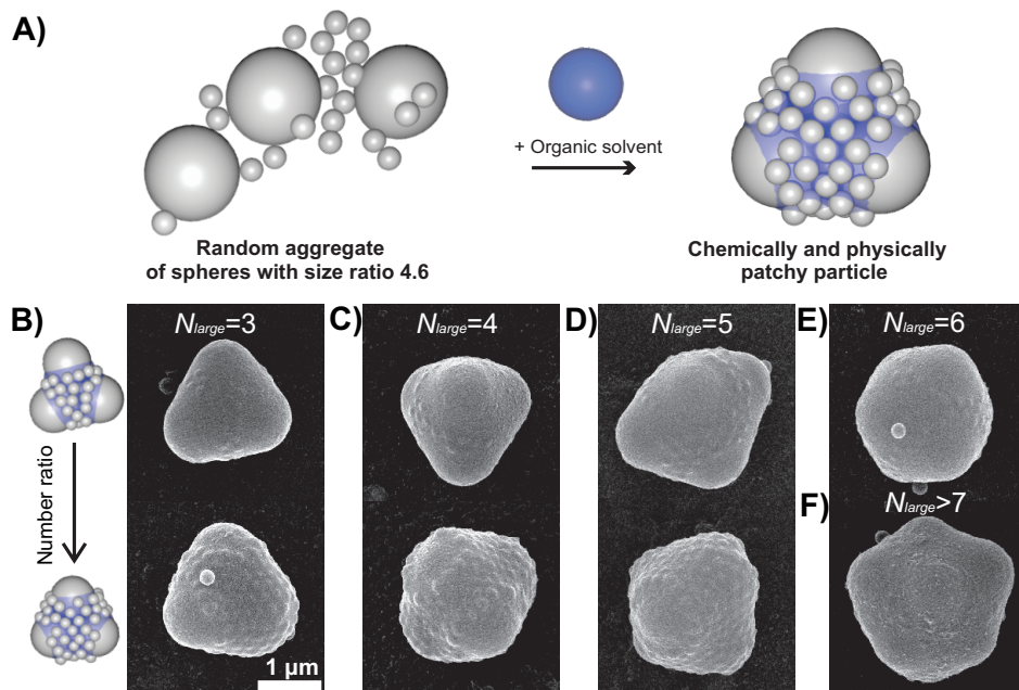
FIGURE 5.6: Chemically and physically patchy particles. A) Illustration of the reconfiguration of an aggregate consisting of spheres with size ratio 4.6. Reconfiguration is induced by the addition of organic solvent. The number of larger spheres, N_{large} , determines the geometry of the patchy particle resulting in the triangle at N_{large}=3 , the tetrahedron at N_{large}=4 , the triangular dipyramid at N_{large}=5 and the octahedron at N_{large}=6 . The small particles position at the contact areas of the larger spheres and determine the final shape of the patchy particle. At large number ratios, the small particles arrange in an hexagonal pattern forming a 'jacket' around the cluster of 1.06 \mu\text{m} spheres. Since the protruding particles introduce surface roughness, the patchy particles own both chemical and physical patchiness.
