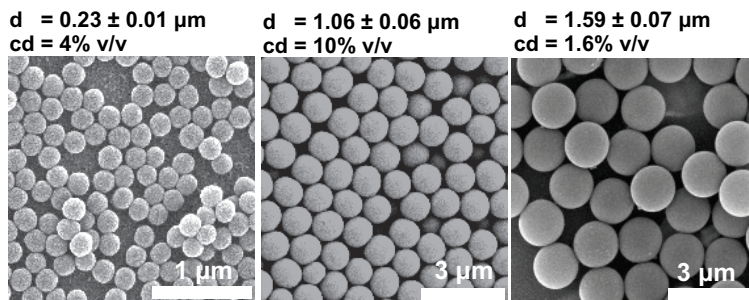
FIGURE 5.1: SEM micrographs of the polystyrene seed particles used in this study. The diameter and crosslink density are listed above the images.
