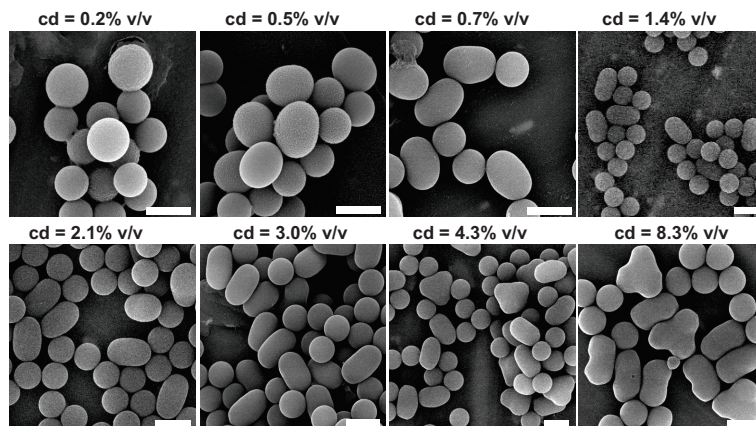
FIGURE 4.8: Typical dumbbells shaped from seed particles with different crosslink densities. The cd of the seeds is stated above the SEM micrographs and the scalebars are 2\ \mu\text{m} . The images indicate that similar shapes were formed and as the crosslink density increases the shape of the original seed particles is more preserved, which is confirmed by a quantitative analysis.
