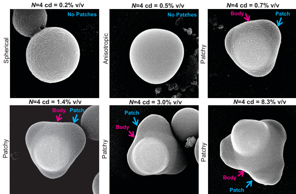
FIGURE 4.4: Spherical, anisotropic and patchy particles shaped from four seed particles. The shape of the cluster after reconfiguration was influenced by the crosslink density ( cd ) of the seed particles. At low crosslink density, cd=0.2\% v/v the seeds merged yielding larger spheres. At cd=0.5\% v/v anisotropic shapes were obtained but no patches were recognized. At cd \geq 0.7\% v/v patchy particles were formed where part of the original seeds can be recognized and distinguished by contrast from the polymerized droplet spanning the sphere, the body. At increasing crosslink density the contrast difference between the patches and the body became larger, making the interface between the two increasingly visible. At cd > 3.0\% v/v the patches could also be distinguished from the body by a difference in the surface morphology of the patches and the body. The patches had small irregular features, which were not visible on the body of the patchy particle.
