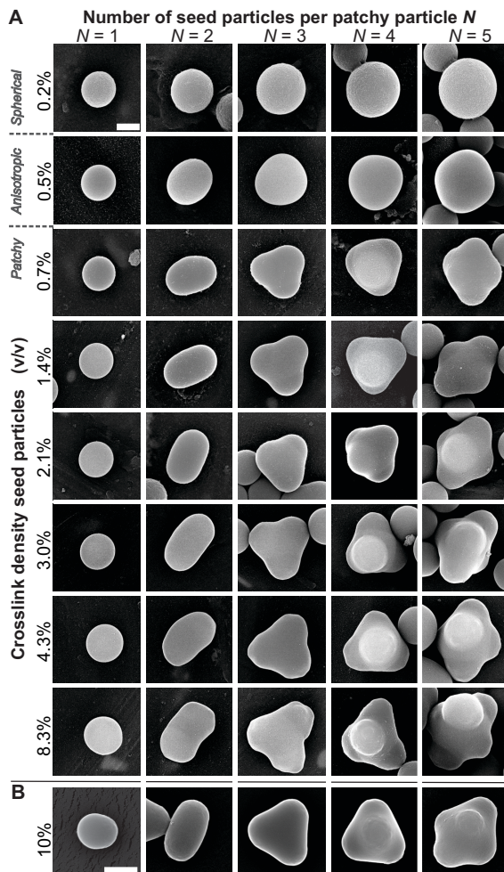
FIGURE 4.3: SEM micrographs of spherical, anisotropic and patchy particles of N=1-5 formed by polystyrene seed particles of different crosslink density (cd). Scale bar is 1\ \mu\text{m} . A) Particles constructed by spheres of fixed crosslink density, ranging from 0.2\% \text{ v/v} at the top row to 8.3\% \text{ v/v} at the bottom row. The seeds are all synthesized following the same emulsion polymerization protocol. Per column particles consisting of a fixed number of seed particles are shown. At 0.2\% \text{ v/v} cd the seed particles completely merge during reconfiguration, which yields spheres with a larger diameter. Spheres with 0.5\% \text{ v/v} cd slightly resist deformation, resulting in anisotropic particles. At higher cd, 0.7 \leq \text{cd} \leq 8.3\% \text{ v/v} , the shape of the seeds is largely preserved and patchy particles are formed. Spheres with very densely crosslinked polymer networks, 4.3 or 8.3\% \text{ v/v} cd, form patchy particles with irregular features at the patches. B) Patchy particles constructed from 10\% \text{ v/v} crosslinked 1.06\ \mu\text{m} seed particles purchased from Magsphere Inc. Large field of view SEM micrographs of the reconfigured particles are shown in Figure 4.5.
