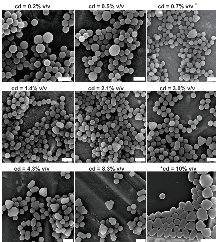
FIGURE 4.5: SEM micrographs of particles obtained by reconfiguring colloidal aggregates of seeds with different crosslink density (cd). The cd of the seeds is stated above the images and the scalebars are 3 \mu\text{m} . The images show typical overviews of the particles observed in the colloidal dispersions. As the crosslink density increases the shape of the original seed particles was more preserved. *The colloids with \text{cd} = 10\% \text{ v/v} were purchased from Magsphere Inc. and synthesized according to a different method compared to the other seed particles.
