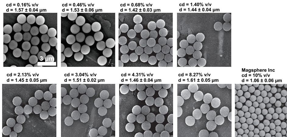
FIGURE 4.1: SEM micrographs of the seed particles used. The crosslink density (cd) and diameter (d) of the particles in the dispersion are stated above the representative images.
