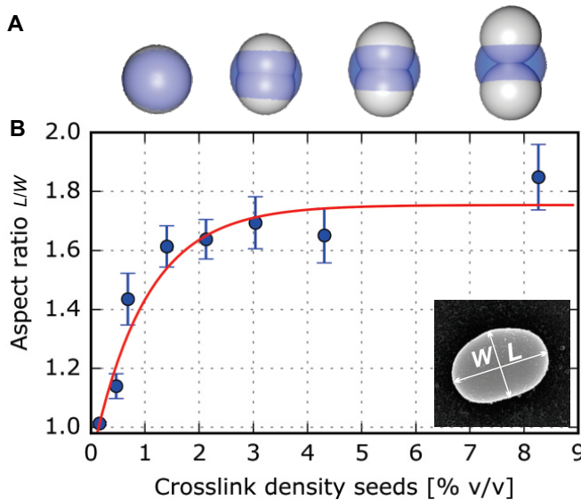
FIGURE 4.7: Deformation of dumbbells. A) Illustration of the effect of capillary forces on the shape of dumbbells constructed from deformable spheres. Sphere deformability decreases from left to right. B) The aspect ratio, L/W , of dumbbells increases with the crosslink density of the seeds. This indicates that the seed particles are less deformed upon reconfiguration at increasing rigidity. The red line is the result of a least squares fit of the data, y = 1.75 - 0.87 \cdot \exp(-cd/1.00) .
