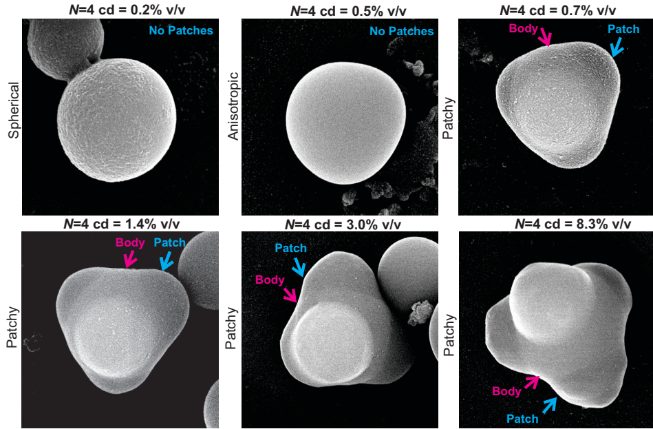
FIGURE 4.4: Spherical, anisotropic and patchy particles shaped from four seed particles. The shape of the cluster after reconfiguration was influenced by the crosslink density (cd) of the seed particles. At low crosslink density, cd=0.2\% v/v the seeds merged yielding larger spheres. At cd=0.5\% v/v anisotropic shapes were obtained but no patches were recognized. At cd \geq 0.7\% v/v patchy particles were formed where part of the original seeds can be recognized and distinguished by contrast from the polymerized droplet spanning the sphere, the body. At increasing crosslink density the contrast difference between the patches and the body became larger, making the interface between the two increasingly visible. At cd > 3.0\% v/v the patches could also be distinguished from the body by a difference in the surface morphology of the patches and the body. The patches had small irregular features, which were not visible on the body of the patchy particle.
