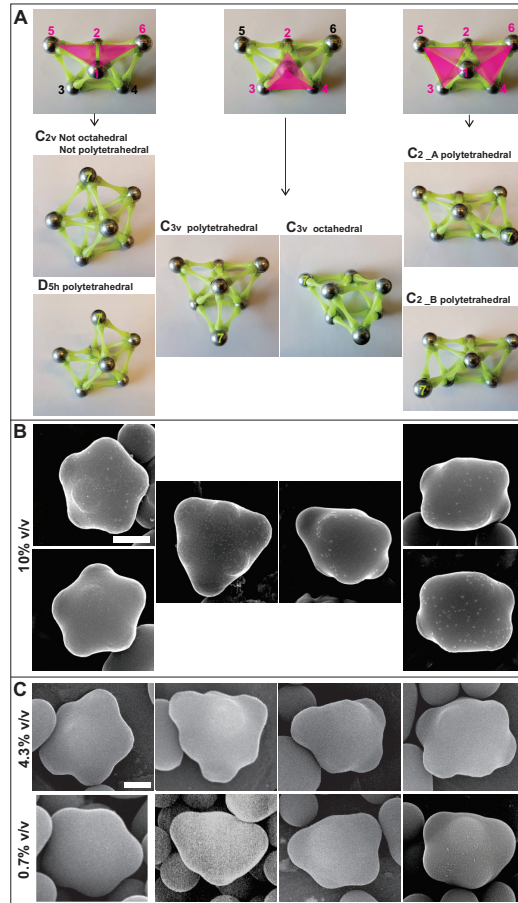
FIGURE 4.10: A) Models of typical minimal free energy geometries for clusters of N=7 . The Schönflies notation is written above the image. Above the N=7 models a polytetrahedron is shown with in magenta the position where the seventh sphere can be positioned to form the N=7 structures. The pentagonal dipyramids C_{2v} and D_{5h} can be differentiated by the subtle bond distance between the two spheres on the pentagon, 1.09d vs 1.05d , respectively, where d is the diameter of the sphere. C_{3v} has a polytetrahedral and an octahedral version. The polytetrahedral C_2 geometry knows two chiral enantiomers. B) and C) SEM images of patchy particles constructed from seven spheres of different crosslink density. Scalebars are 1\ \mu\text{m} . B) For patchy particles of spheres with 10% v/v crosslink density, purchased from Magsphere Inc., all six N=7 geometries can be identified and these rigid spheres predominantly reconfigure into the pentagonal dipyramid geometries ( C_{2v} and D_{5h} ). C) Patchy particles with a cd of 4.3% v/v reconfigure into all geometries although we were unable to distinguish between the C_{2v} and D_{5h} geometry and only one C_2 structure is shown. At low crosslink density, 0.7% v/v, the pentagonal dipyramids C_{2v} and D_{5h} are rarely observed.
