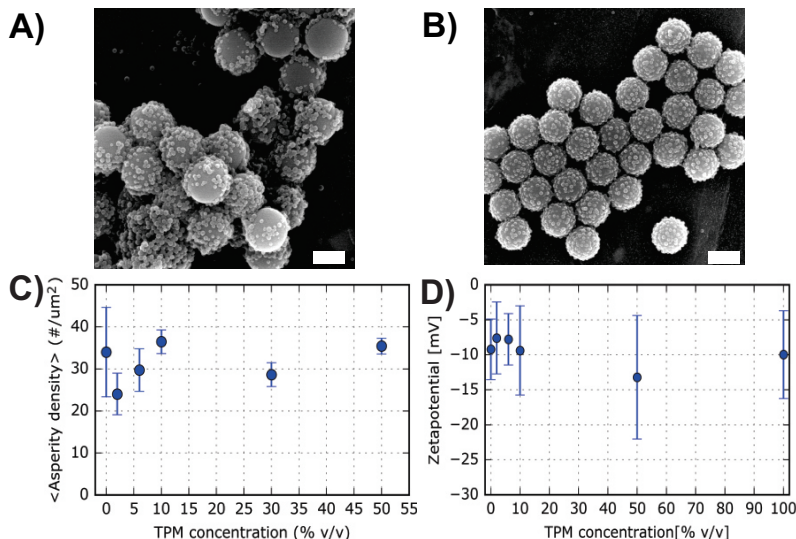
FIGURE 2.4: Surface roughness uniformity and stabilization for colloids swollen with [\text{TPM}] \leq 50\% \text{ v/v} . Scalebar is 1 \mu\text{m} . A-B) SEM micrographs of LPS colloids swollen in the absence of HQ. A) Rough colloids obtained by swelling with 100\% \text{ v/v} styrene. The asperities on these colloids are non-uniformly distributed on the surface. (B) Rough stable colloids were formed by swelling with a styrene:TPM \text{v/v} ratio of 50:50. The particle surface is uniformly covered with asperities. C) The spread in the distribution of asperities on the surface of the particles decreases with the TPM concentration. D) Zetapotential values of polystyrene-TPM hybrid colloids, obtained by swelling with styrene:TPM ratios of 100:0 to 0:100. The zetapotential is not sufficient to contribute electrostatically to the stabilization of the colloids.
