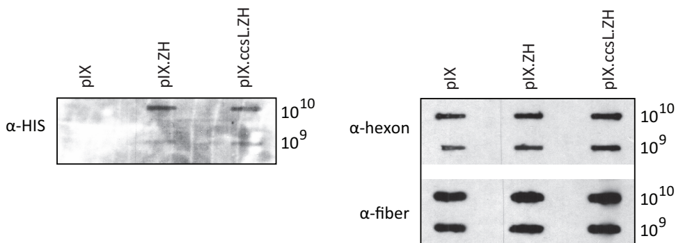
Figure 2 Slot-blot analyses of HER2-ECD binding to intact virus particles. HER2-ECD binding was assayed by subsequent incubation with his-tagged HER2-ECD and anti-HIS antibody. For loading-control purpose, incubation with anti-fiber-knob and anti-hexon antibody was performed. Two virus concentrations (10 10 and 10 9 pp) were applied to the membrane.
