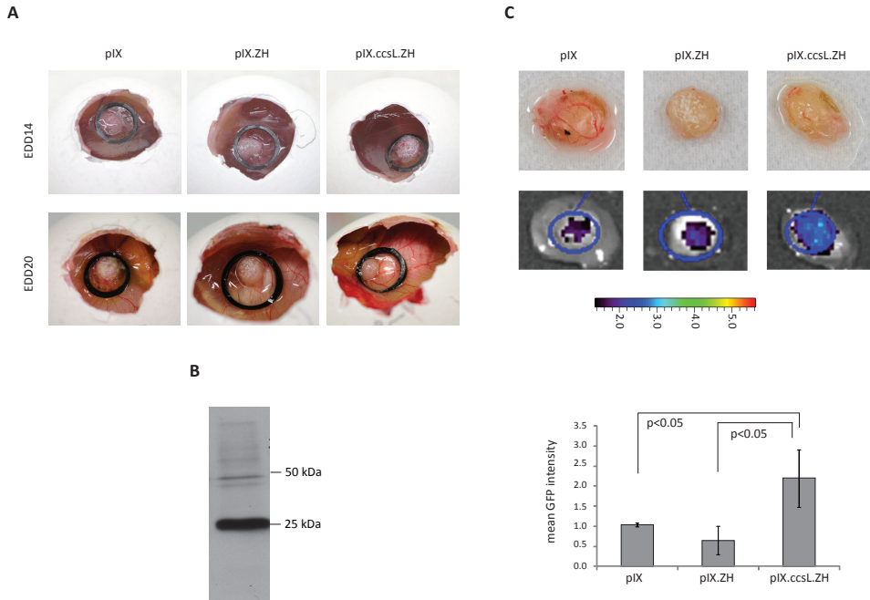
Figure 4 Virus transduction of SKOV-3 cells grown on the CAM. (a) Representative pictures of CAM tumours at EDD 14 (before virus injection) and EDD 20 (before tumour isolation). (b) Western analysis of cathepsin L protein levels in lysates of SKOV-3 cells grown as CAM tumour. Detection was carried out with anti-cathepsin L antibody directed against pro-cathepsin L (42 kDa) as well as the active form of cathepsin L (25 kDa). (c) Biofluorescent imaging with the IVIS system of GFP expression in SKOV-3 tumours retrieved from the CAM (EDD 20). The graph shows the mean GFP intensities. Error bars represent s.d. (n = 5). Representative IVIS pictures are included.
