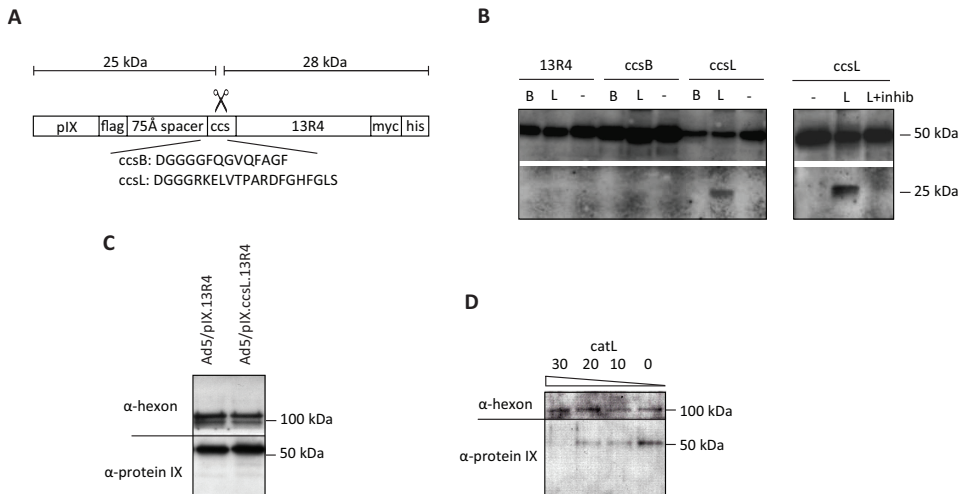
Figure 1 (a) Schematic representation of the pIX.13R4 fusion proteins. All polypeptide components are indicated (protein IX, flag tag, 75-Ångstrom spacer, ccs, 13R4 (single-chain antibody fragment directed against β-galactosidase), myc tag, his tag). (b) Western analyses after cathepsin cleavage of pIX.13R4 fusion proteins bound to nickel beads. The left panel indicates pIX.13R4 (13R4), pIX.ccsB.13R4 (ccsB) and pIX.ccsL.13R4 (ccsL) protein levels after cathepsin B (catB), cathepsin L (catL) or mock incubation. The right panel indicates pIX.ccsL.13R4 protein levels after cathepsin L cleavage in the presence or absence of the cathepsin inhibitor Z-FY(t-Bu)-DMK. Analyses were performed using anti-protein IX antibody. (c) Western analysis of pIX.13R4 and pIX.ccsL.13R4 protein levels after incorporation in the capsid of the protein IX-deleted HAdV mutant dl313 (5 x 10 9 pp per lane). Detection was carried out with anti-protein IX and anti-hexon antibodies. (d) Western analysis of pIX.ccsL.13R4 incorporated in the dl313 virus after incubation with different concentrations of cathepsin L (0, 10, 20 and 30 ng μl -1 ) (5 x 10 9 pp per lane). Detection was carried out with anti-protein IX and anti-hexon antibodies.
