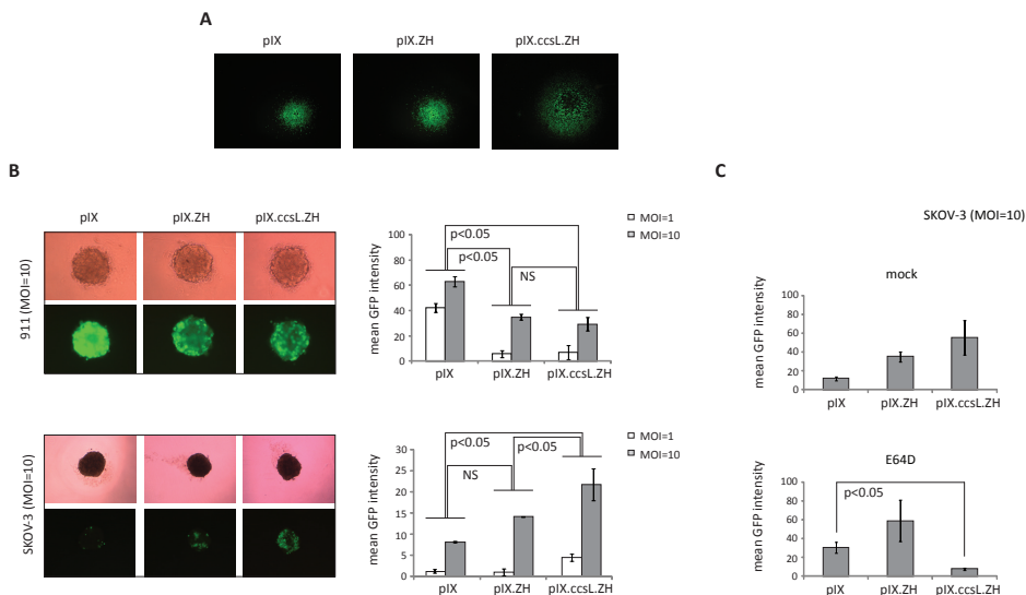
Figure 3 (a) Plaque assay to compare Ad5/pIX, Ad5/pIX.ZH and Ad5/pIX.ccsL.ZH infection of monolayer cell cultures. The microscopy pictures show representative GFP-positive SKOV-3 plaques. (b) Transduction of 911 and SKOV-3 spheroids with Ad5/pIX, Ad5/pIX.ZH and Ad5/pIX.ccsL.ZH. Infection was performed at multiplicities of infection (MOI) of 1 and 10 PFU per cell. The graphs show the mean GFP intensities at 5 days post-transduction. Error bars represent s.d. ( n = 3 ). Differences in GFP intensity are considered significant at P < 0.05 for both MOIs. Representative pictures (at 5 days post-transduction) are shown on the left. (c) Transduction of SKOV-3 spheroids with Ad5/pIX, Ad5/pIX.ZH and Ad5/pIX.ccsL.ZH in the presence or absence of the cysteine protease inhibitor E64-D. The graphs show the mean GFP intensities at 5 days post-transduction. Error bars represent s.d. ( n = 3 ).
