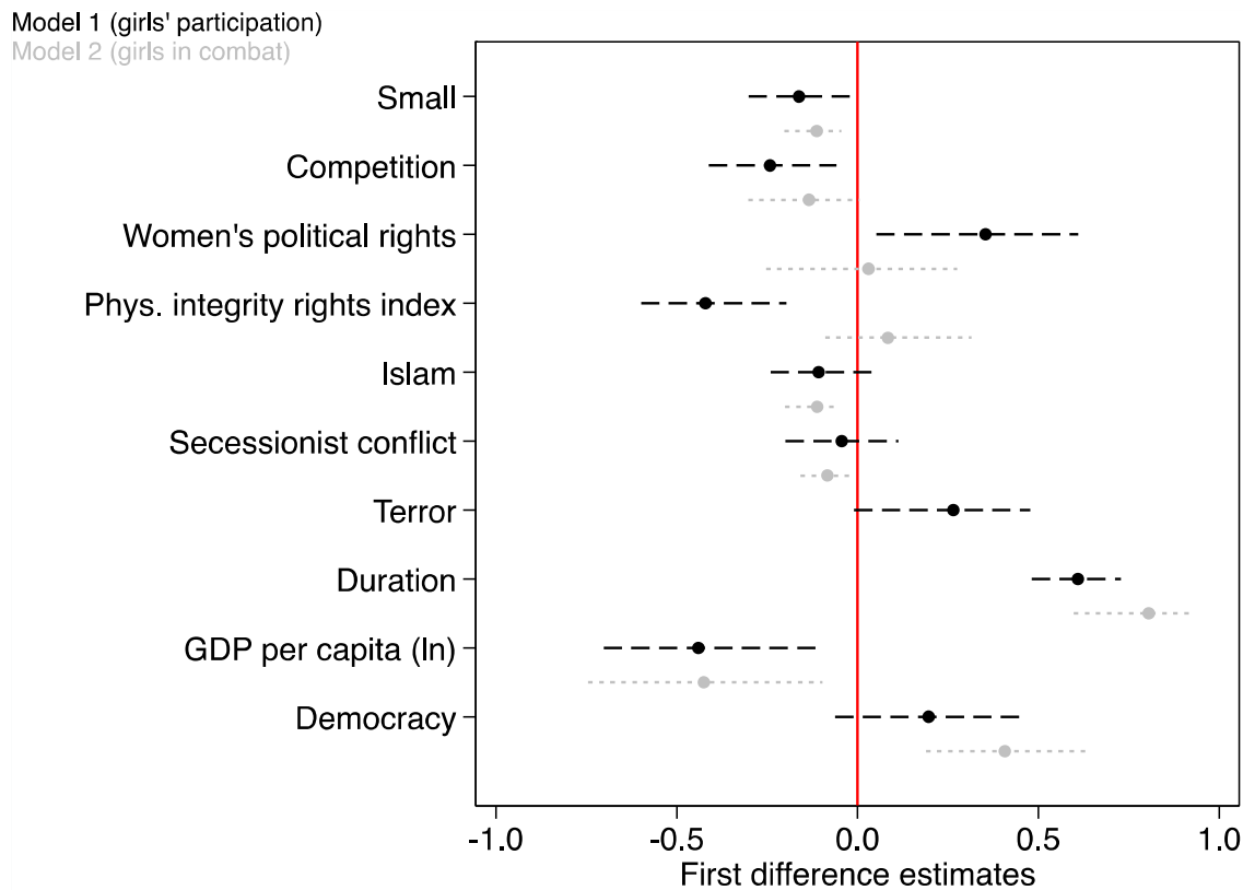
Figure 2. First differences
