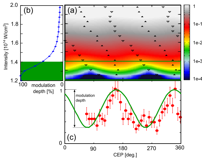
FIG. 3 (color online). Comparison of simulated and measured fragmentation probability of the channel \text{C}_2\text{H}_2^+ \rightarrow \text{CH}^+ + \text{CH}^+ . (a) Simulated fragmentation probability encoded in color scale as a function of CEP and laser intensity, normalized to its maximum value and calculated as described in the Supplemental Material [10]. The CEP and intensity dependent position of maximum and minimum fragmentation yield is indicated by black upwards and gray downwards pointing triangles, respectively. (b) Modulation depth of the fragmentation probability [as defined in (c)], as a function of laser intensity. (c) Simulated fragmentation probability over CEP (full green line) obtained by averaging of the data in (a) over the intensity range 1.2\text{--}1.4 \times 10^{14} \text{ W/cm}^2 to account for the experimental intensity beam profile [as indicated in (a) and (b)], in comparison with the experimental data from Fig. 1(a) shifted by 60^\circ .
