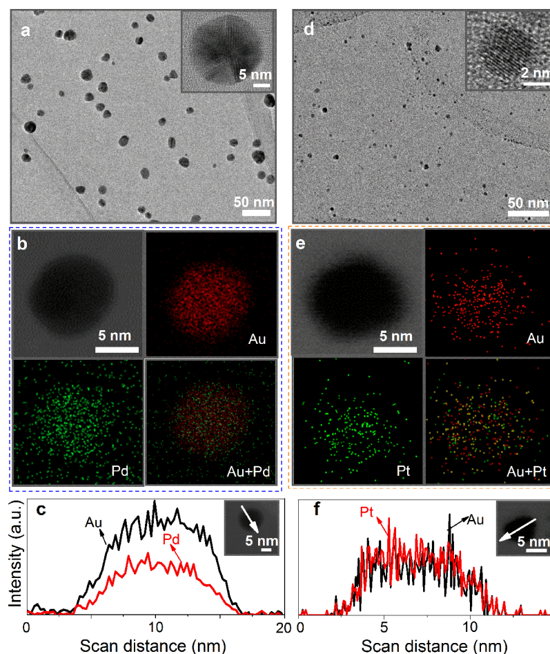
Figure 3. Composition analysis of nanoalloys generated by cathodic corrosion. TEM (a, d)/HRTEM images (insets in (a) and (d)), scanning TEM (STEM) images, element mapping analysis (b, e), and line scan profiles (c, f) of randomly selected Pd–Au (a–c) and Pt–Au alloy NPs (d–f). In the elemental mapping, Au is color-coded red, whereas Pt and Pd are marked as green.
