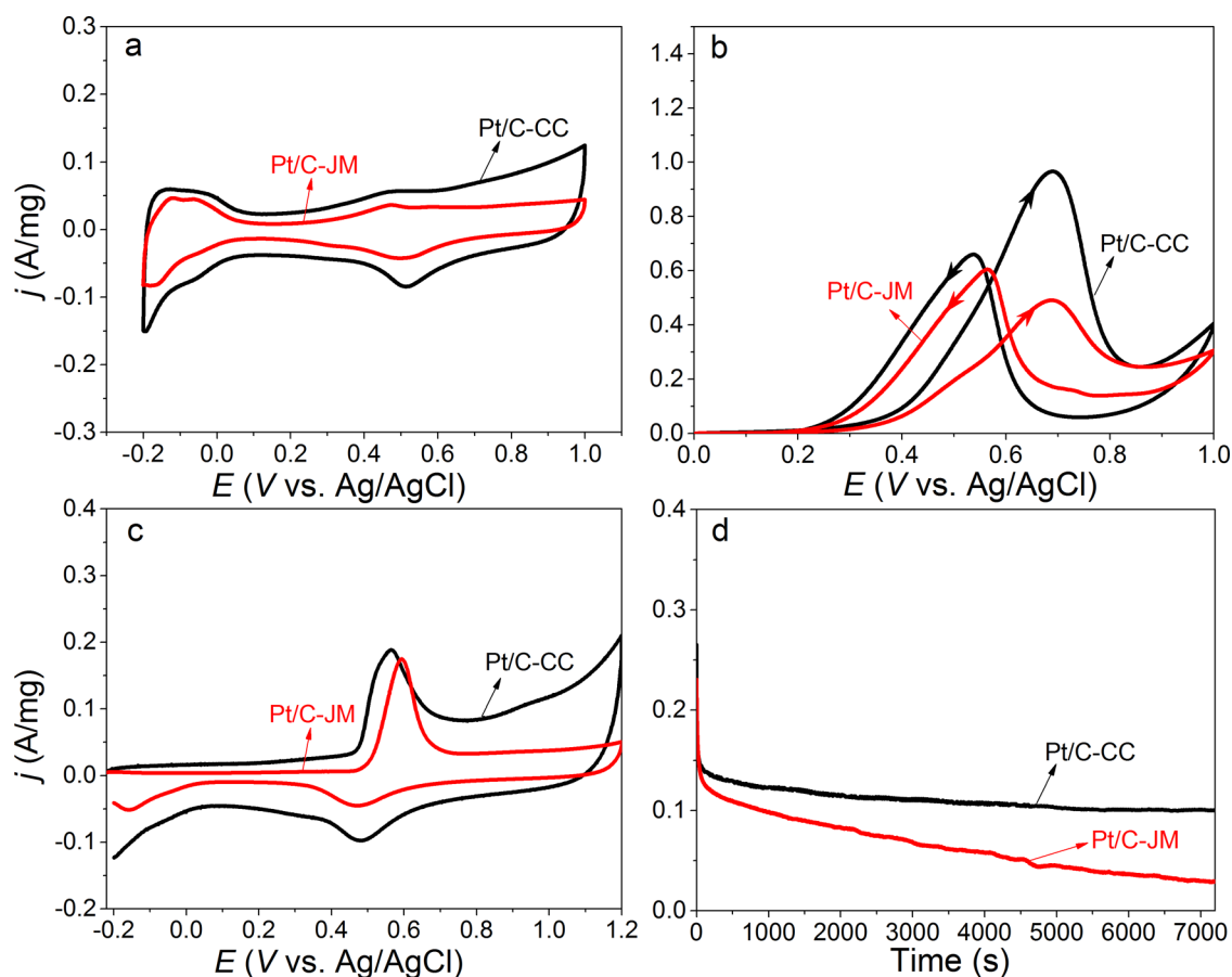
Figure 2. Cyclic voltammograms (CVs) of Pt/C-CC and Pt/C-JM catalysts in 0.1 M HClO 4 at a scan rate of 50 mV/s (a) and in 0.1 M HClO 4 and 1.0 M CH 3 OH at a scan rate of 20 mV/s (b). CO stripping voltammograms (c) of Pt/C-CC and Pt/C-JM catalyst in 0.1 M HClO 4 at a scan rate of 50 mV/s. Chronoamperograms (d) at 0.45 V of Pt/C-CC and Pt/C-JM catalyst in 0.1 M HClO 4 and 1.0 M CH 3 OH. The current density in the CVs is normalized by the respective mass of Pt loading.
