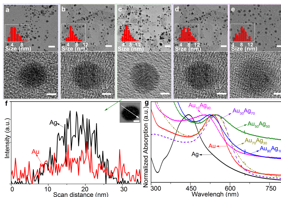
Figure 4. Analysis and characterization of AuAg nanoalloys. TEM images of Au 90 Ag 10 , Au 70 Ag 30 , Au 50 Ag 50 , Au 30 Ag 70 , and Au 10 Ag 90 nanoalloys (a–e). Particle size distributions are added as insets of the TEM images in the first row (scale bar 20 nm) and the corresponding HRTEM images (scale bar 2 nm) are assembled in the second row. (f) Line scan profiles of Au 50 Ag 50 nanoalloys with STEM image (inset, scale bar 5 nm); UV–vis absorption spectra of monometallic (Au, Ag) NPs and the Ag x Au 100–x nanoalloys (g).
