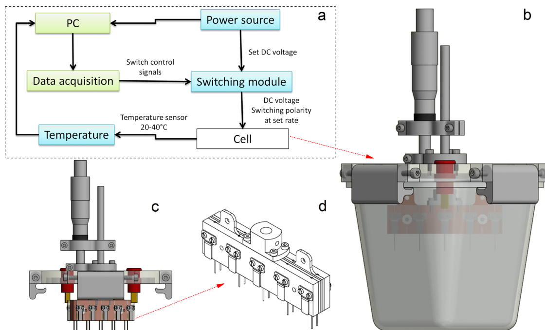
Figure 5. Schematic illustration of the “comb-electrode” setup. The block diagram of the global design of the setup (a), the complete cell system (b), the electrode feeding component (c), and an enlarged comb consisting of five electrode pairs (d). A micrometer screw mounted on the comb electrodes was used to precisely adjust their submersion depth (measured from the moment the electrode touches the liquid surface) in the liquid.
