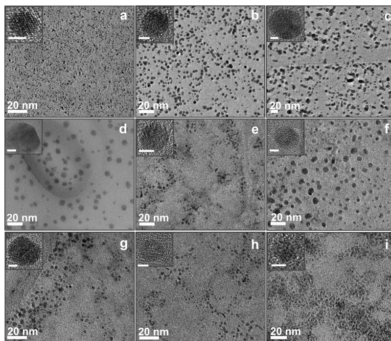
Figure 1. TEM/HRTEM images. All of the insets in the upper left corner have a scale bar of 2 nm, whereas all of the main figures have a scale bar of 20 nm. Pt NPs produced in 0.1 M NaOH (a), Au NPs produced in 1 M \text{Ca}(\text{NO}_3)_2 (Au-I) (b), Au NPs produced in 0.3 M \text{Na}_2\text{SO}_4 (Au-II) (c), Ag NPs produced in 0.1 M NaOH (d), Pd NPs produced in 0.3 M \text{CaCl}_2 (e), Rh NPs produced in 0.3 M \text{CaCl}_2 (f), Ir NPs produced in 0.3 M \text{CaCl}_2 (g), Cu NPs produced in 0.3 M \text{CaCl}_2 (h), and Ni NPs produced in 0.3 M \text{Na}_2\text{SO}_4 (i). All of the bulk wires were treated at \pm 10 V with a square waveform at a frequency of 100 Hz and were submerged in various electrolyte solutions with 5 wt % PVP. According to our empirical experience and earlier work, 23 different electrolytes were chosen for different metals to guarantee efficient NP production. Here, using the positive voltage is essential to facilitate the detachment of NPs from the electrode surface. 23
