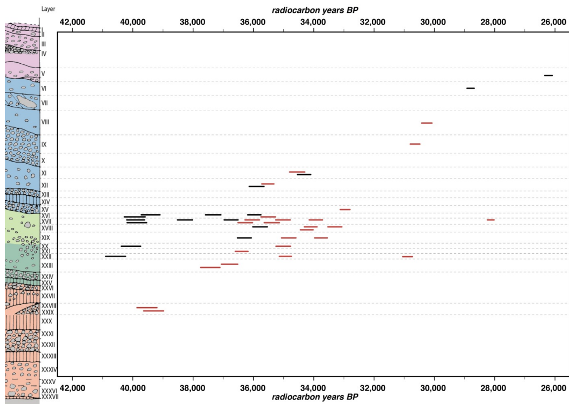
Figure 4.2: Radiocarbon determinations by Douka et al. 2013 (red) and Bosch et al. 2015a (black) for Ksâr 'Akil sorted by layer. Results show a one-sigma range (uncal BP).
