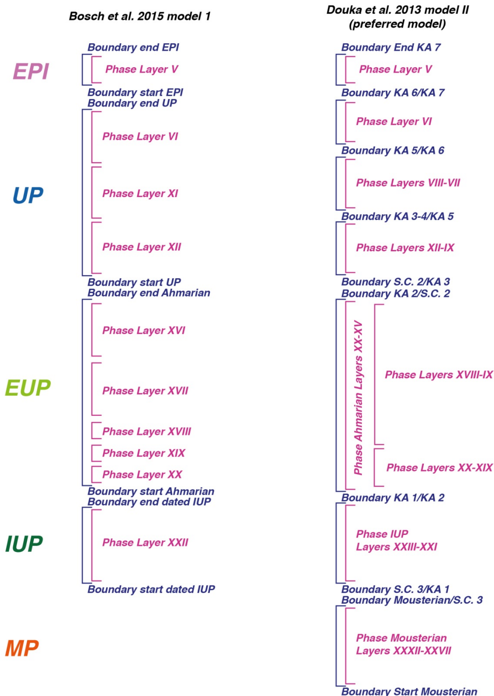
Figure 4.1: Schematic of the Bayesian models of Bosch et al. (2015a) and Douka et al. (2013) showing the placement of boundaries (blue) and phases (pink). The models used are Bosch et al.'s (2015a) Model 1 and Douka et al.'s (2013) preferred Bayesian Model II. Left column shows technocomplexes at Ksâr 'Akil as used by Bosch et al. (2015a). Abbreviations: MP: Middle Palaeolithic, IUP: Initial Upper Palaeolithic, EUP: Early Upper Palaeolithic (Early Ahmarian), UP: Upper Palaeolithic, EPI: Epipalaeolithic. Abbreviations used in Boundary and Phase labels after Bosch et al. (2015a) and Douka et al. (2013).
