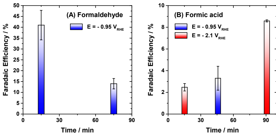
Figure A.3 Faradaic efficiency towards (A) formaldehyde and (B) formic acid at E = -0.95 \text{ V}_{\text{RHE}} and E = -2.1 \text{ V}_{\text{RHE}} on BDD in 0.001 M \text{HClO}_4 + 0.099M \text{NaClO}_4 electrolyte
