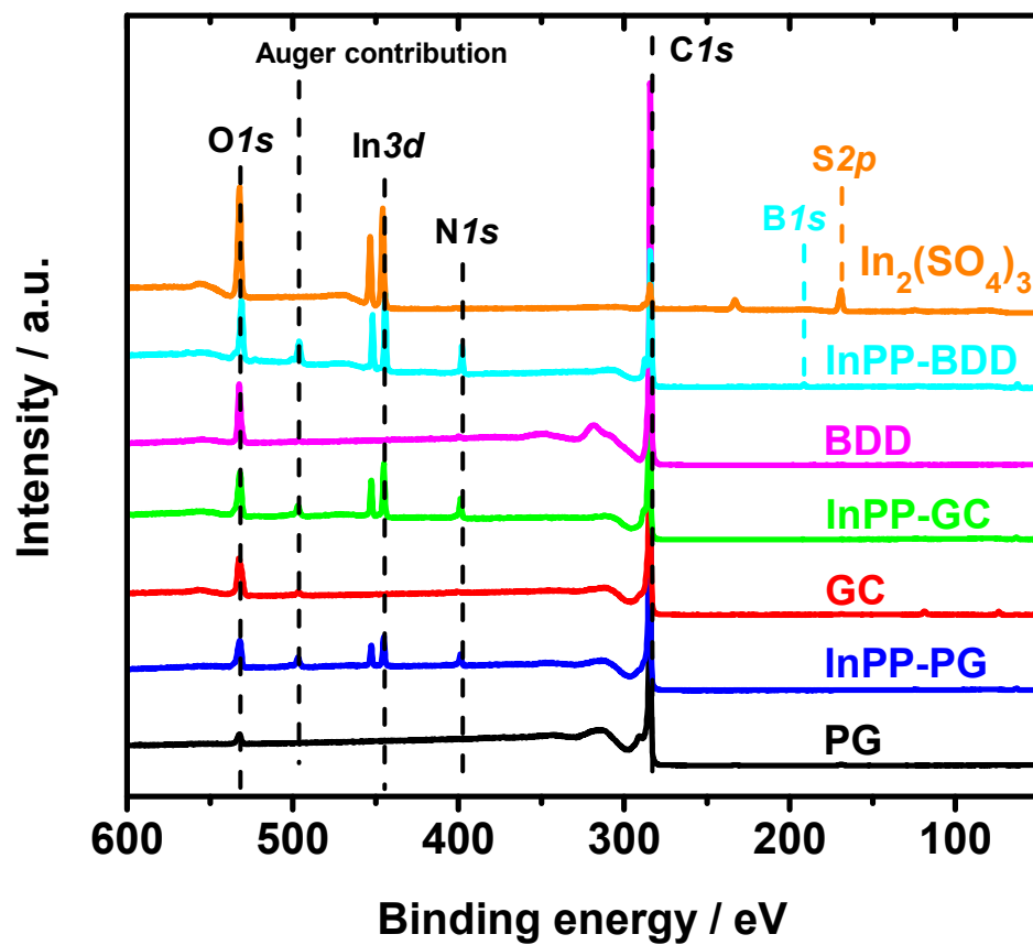
Figure C.12 XPS spectra of the different substrates with and without immobilized InPP, and In 2 (SO 4 ) 3 .
