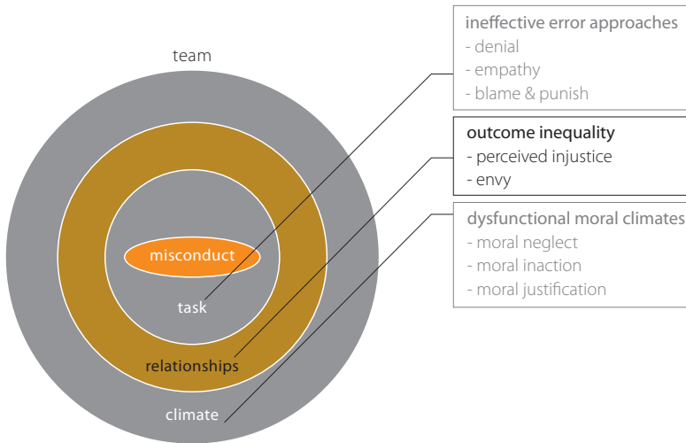
Figure 8.6. Outcome inequality
