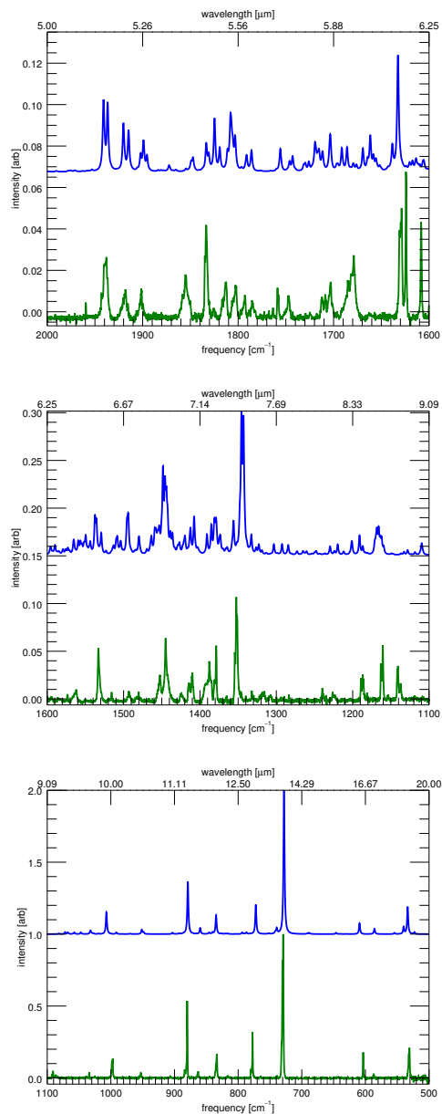
Figure 5.9 The matrix–isolation infrared spectrum[36, 79] of 9–methylanthracene (green, bottom of each panel) compared to the convolved (FWHM 2 \text{cm}^{-1} ) theoretical anharmonic calculations of this work (blue, top each panel). Three spectral ranges are shown, with each range normalized to the local maximum to enhance details.
