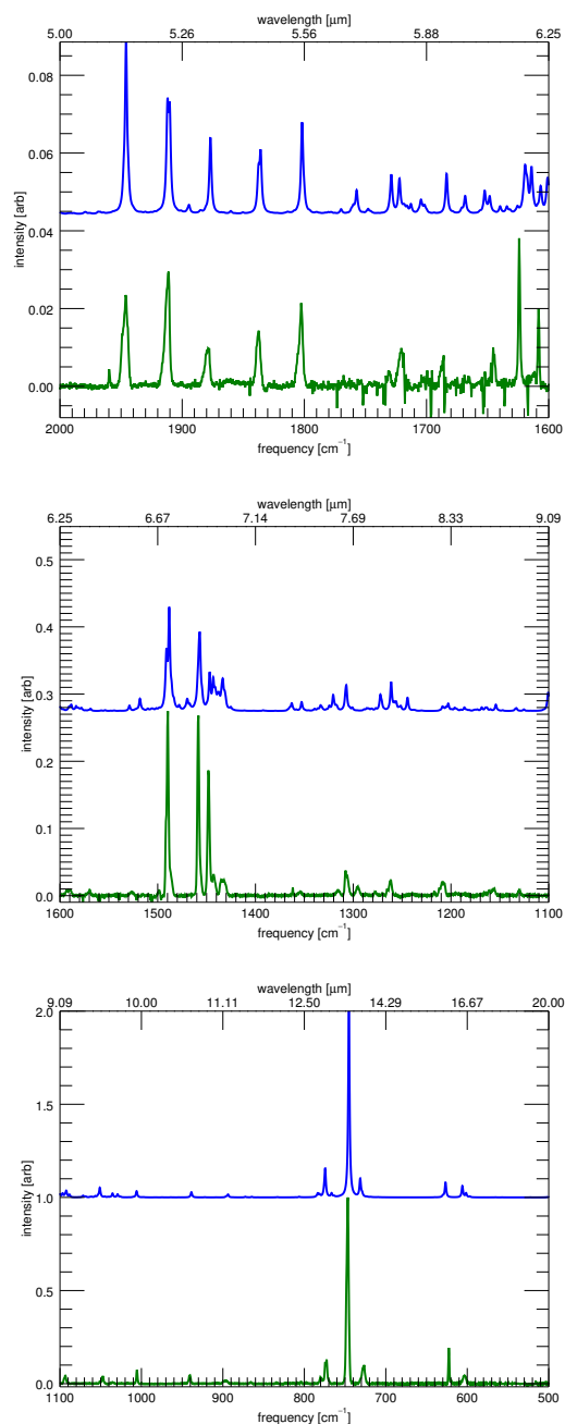
Figure 5.3 The matrix-isolation infrared spectrum[36, 79] of 9,10-dihydrophenanthrene (green, bottom of each panel) compared to the convolved (FWHM 2 cm -1 ) theoretical anharmonic calculations of this work (blue, top each panel). Three spectral ranges are shown.
