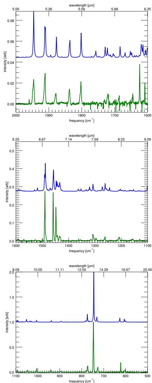
Figure 5.3 The matrix-isolation infrared spectrum[36, 79] of 9,10-dihydrophenanthrene (green, bottom of each panel) compared to the convolved (FWHM 2 cm -1 ) theoretical anharmonic calculations of this work (blue, top each panel). Three spectral ranges are shown.
