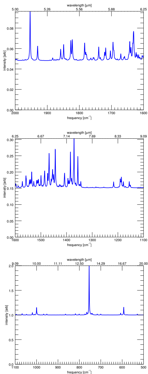
Figure 5.11 No matrix-isolation data is available for 9,10-dimethylantracene. Therefore, only the convolved (FWHM 2\text{ cm}^{-1} ) theoretical anharmonic calculations of this work (blue, top each panel). Three spectral ranges are shown, with each range normalized to the local maximum to enhance details.
