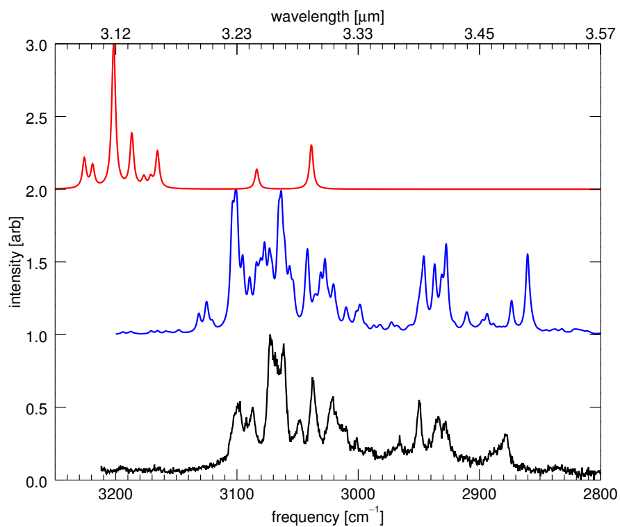
Figure 1.4 Three infrared spectra of the C–H stretching region of 9-methylantracene: The harmonic spectrum (red, top), anharmonic spectrum (blue, middle), and the high-resolution experimental spectrum (black, bottom).
