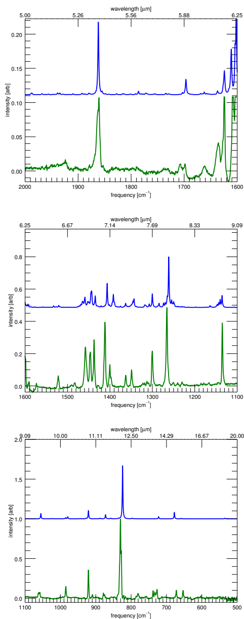
Figure 5.19 The matrix-isolation infrared spectrum[36, 79] of 1,2,3,6,7,8-hexahydropyrene (green, bottom of each panel) compared to the convolved (FWHM 2 cm -1 ) theoretical anharmonic calculations of this work (blue, top each panel). Three spectral ranges are shown, with each range normalized to the local maximum to enhance details.
