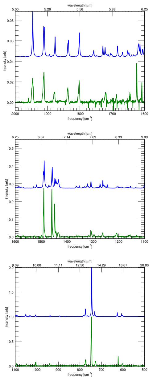
Figure 5.15 The matrix-isolation infrared spectrum[36, 79] of 9,10-dihydrophenanthrene (green, bottom of each panel) compared to the convolved (FWHM 2 cm -1 ) theoretical anharmonic calculations of this work (blue, top each panel). Three spectral ranges are shown, with each range normalized to the local maximum to enhance details.
