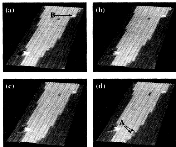
FIG. 1. Sequence of four STM images of the Au(110) surface ( 160 \text{ \AA} \times 513 \text{ \AA} , V_t = -0.88 \text{ V} , I_t = 0.1 \text{ nA} ) measured at 375 \text{ K} at a rate of 1 image/49 s.
