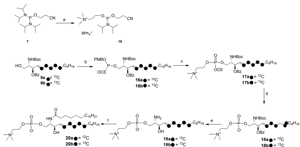
Scheme 4.2 Synthesis of ( 13 C 5 -labeled) sphingosine 1-cholinephosphate 19a/b and sphingomyelins 20a/b .
