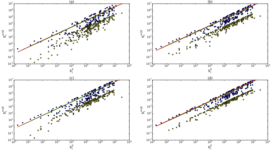
Figure 3.3: Strength of layer \beta versus inter-layer multiplexed strength for 4 different pairs of commodities: inorganic chemicals (a), plastics (b), iron and steel (c), electric machinery (d) versus trade in cereals. Blue dots: real data; yellow dots: expected multiplexed strength according to the uncorrelated model; lower green line: expected trend according to (3.59); upper red line (when discernible): best fit. In all the cases, R^2 > 0.92 , for both the curves. It should be noted that we fit the empirical data with lines of the form y = a \cdot x , and only after we plot the results in log-log scale.
