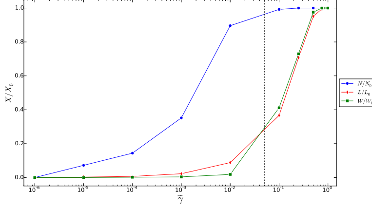
Figure 4.15: Effect of filtering on the Florida Bay food web dataset. We report the fraction of the number of nodes N/N_0 (blue dots), edges L/L_0 (red diamonds) and total weight W/W_0 (green squares) as a function of the p -value \tilde{\gamma} . The vertical line corresponds to \tilde{\gamma} = 0.05 .
