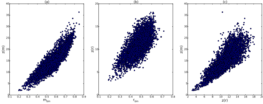
Figure 2.4: Analysis of significance of the values of binary multiplexity and multireciprocity for the WTM. Left: binary transformed multiplexity \mu_b^{\alpha\beta} versus its corresponding z -score z(m_b^{\alpha\beta}) ; center: binary transformed multireciprocity \rho_b^{\alpha\beta} versus its corresponding z -score z(r_b^{\alpha\beta}) ; right: z(r_b^{\alpha\beta}) vs z(m_b^{\alpha\beta}) . Only off-diagonal values are reported.
