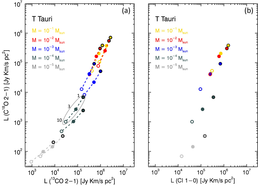
Figure 3.14: Line luminosity of \text{C}^{18}\text{O} vs ^{13}\text{CO} ( J = 2-1 ) (panel a) and \text{C}^{18}\text{O} vs [CI] ( J = 1-0 ) (panel b) for ten models, run also with a reduced initial atomic C and ^{13}\text{C} abundances. The standard value, X_{\text{C}} = [\text{C}]/[\text{H}] = 1.35 \times 10^{-4} , has been reduced by factors of 3 and 10. The models with ISM-like carbon abundances are shown by the outlined symbols, those with a factor of 3 of carbon depletion by the filled symbols and those with a factor of 10 depletion by the unfilled symbols.
