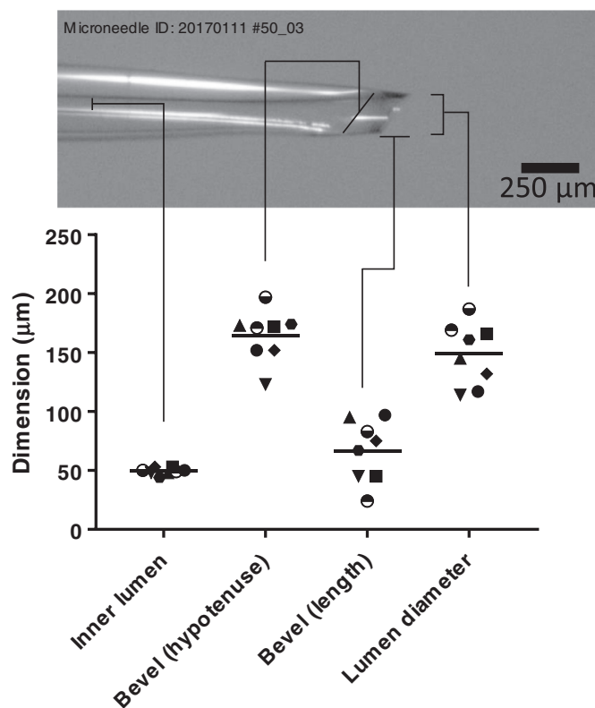
Fig. 2. Representative image of a hollow microneedle produced from a fused silica capillary with an inner lumen diameter of 50 μm (upper image). Dimensions of geometry parameters of 8 individual hollow microneedles, represented by a unique symbol (lower image). The bar represents the geometric mean.
