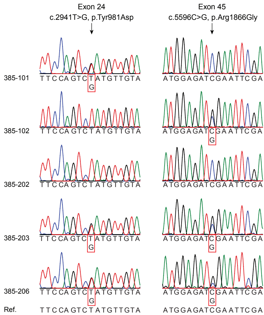
FIGURE 4. Two SMCHD1 variants in trans in Rf385. Sanger sequence tracks from Rf385 family members showing that the two variants are located in trans . Individuals 385-203 and 385-206 carry both SMCHD1 variants (c.2941T>G and c.5596C>G), both indicated with an arrow. Individual 385-101 carries only the SMCHD1 variant in exon 24. Individual 385-102 carries only the SMCHD1 variant in exon 45. Individual 385-202 carries the reference nucleotide for both variants.
