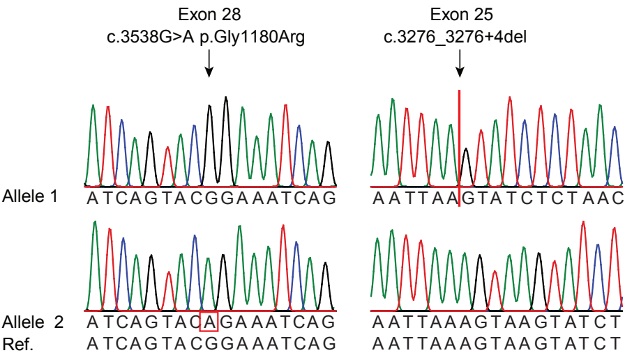
FIGURE 3. Two SMCHD1 variants in trans in Rf1414. Sanger sequence tracks from two clones showing the different SMCHD1 alleles of individual 1414-201. Allele 1 contains the variant in exon 25 (c.3276_3276+4del) and allele 2 contains the variant in exon 28 (c.3538G>A), both indicated with an arrow.
