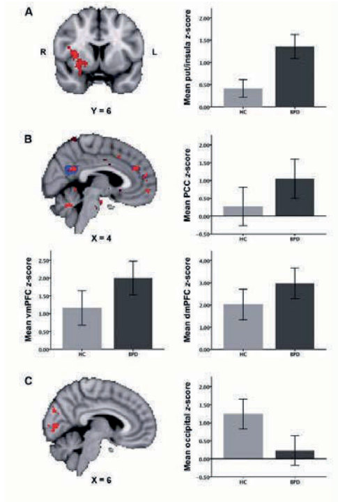
Figure S4.2. Between-group differences in RSFC of each of the three seeds without global signal regression: A) Amygdala (medial temporal lobe network; p < .05 , cluster corrected); B) Dorsal ACC (salience network; p < .001 , uncorrected, overlaid on the original result with global signal regression in blue); C) Ventral ACC (default mode network; p < .05 , cluster corrected). Connectivity differences are overlaid on the MNI 2mm standard space template. Bar graphs plot the mean Z-scores ( \pm 2 SEM) in each group for each of the regions where FC differences are found.
