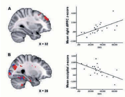
Figure S4.3. Voxel-wise correlations between trait dissociation (DES) and amygdala RSFC without global signal regression in BPD: A) Left amygdala-dlPFC connectivity is positively associated with dissociation ( p < .05 , cluster corrected); B) Left amygdala-occipital cortex FC (including the lingual gyrus, intra-calcarine cortex, and fusiform gyrus) is negatively associated with dissociation ( p < .001 , uncorrected, overlaid on the original result with global signal regression in blue). Results are overlaid on the MNI 2mm standard space template, according to the radiological convention. Scatter plots illustrate the direction of the correlation, with mean Z-scores plotted against DES scores.
