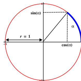
Figure 17.10: The unit circle
