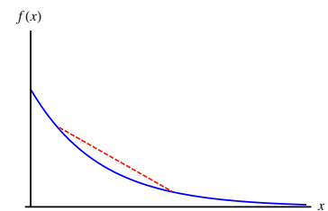
Figure 19.2: Examples of an increasing (top) and a decreasing (bottom) convex function. A line segment connecting any two points on a convex curve will lie above the curve.
