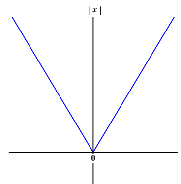
Figure 17.4: Shape of the modulus function.
