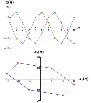
Figure 11.6: Dynamics (top) and phase plot (bottom), for the linear model with \mathbf{A} as in Eq. (11.14), and x_1(0) = 5, x_2(0) = 10 . Top: x_1(n) brown and x_2(n) green.
