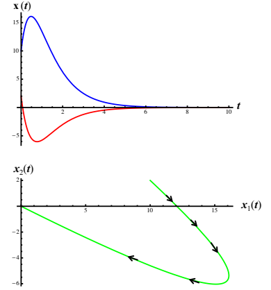
Figure 13.2: Dynamics of the linear model with A given in (13.25) and initial condition (10, 2). Top: x_1(t) (blue) and x_2(t) (red) versus time. Bottom: phase plot.
