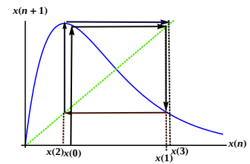
Figure 10.15: Illustration of the cobweb method.
