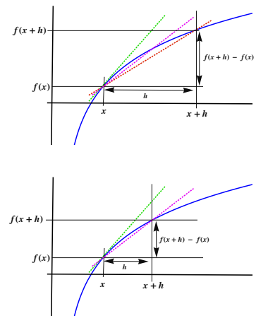
Figure 19.1: The difference quotient and its limit.
