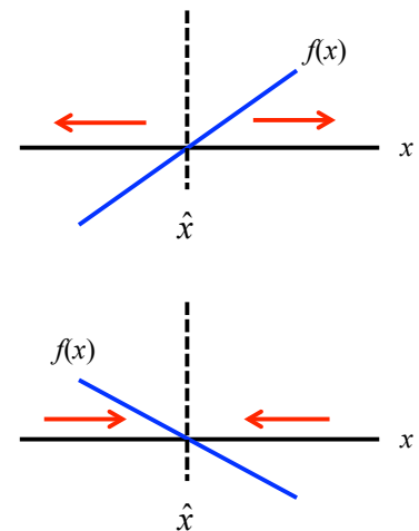
Figure 12.4: Illustration of local stability properties. Blue lines indicate the linear approximation of f(x) , with f'(x) > 0 in top figure, and f'(x) < 0 in bottom figure. Arrows indicate the directions of change in x .
