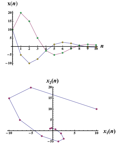
Figure 11.3: Dynamics (top) and phase plot (bottom), for the linear model with \mathbf{A} as in Eq. (11.11), and x_1(0) = 10, x_2(0) = 10 . Top: x_1(n) brown and x_2(n) green.
