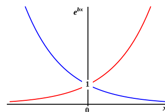
Figure 17.8: Shape of exponential functions. Blue: b < 0 , Red: b > 0
