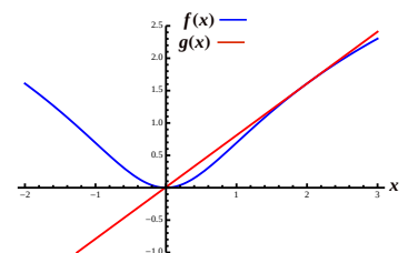
Figure 19.6: Graph of the function in (19.19) and its first order Taylor approximation in the point x = 2 .
