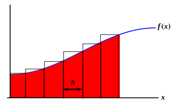
Figure 20.4: Approximation of the surface under the curve.
