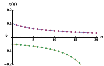
Figure 10.9: Dynamics of the model in (10.34) for two different values of x(0) lying close to the equilibrium, but at different sides.
