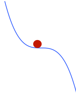
Figure 10.8: A marble in a landscape, at a half stable equilibrium.
