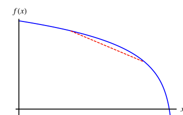
Figure 19.3: Examples of an increasing (top) and a decreasing (bottom) concave function. A line segment connecting any two points on a concave curve will lie below the curve.
