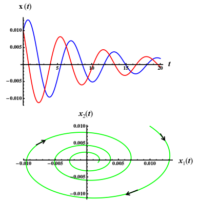
Figure 13.3: Dynamics of the linear model with A given in (13.26) and initial condition (0.01, 0.01). Top: x_1(t) (blue) and x_2(t) (red) versus time. Bottom: phase plot.
