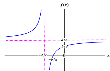
Figure 17.5: Example of the shape of a linear fractional function if ad > cb .
