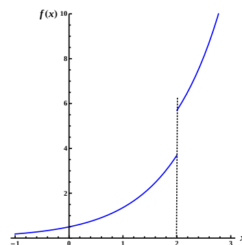
Figure 17.14: Example of a function with a discontinuity at x = 2 .
