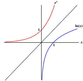
Figure 17.9: The exponential function and the natural logarithm.
