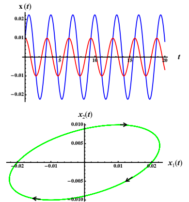
Figure 13.4: Dynamics of the linear model with A given in (13.27) and initial condition (0.01, 0.01). Top: x_1(t) (blue) and x_2(t) (red) versus time. Bottom: phase plot.
