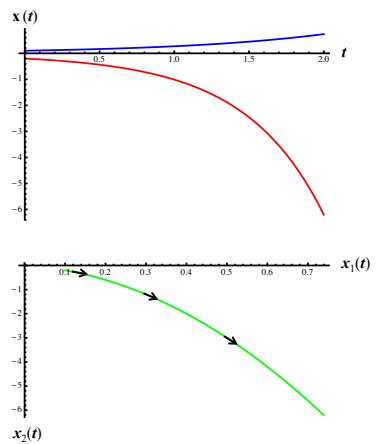
Figure 13.7: Dynamics of the linear model with \mathbf{A} given in (13.29) and initial condition (0.1, -0.2) . Top: x_1(t) (blue) and x_2(t) (red) versus time. Bottom: corresponding phase plot.
