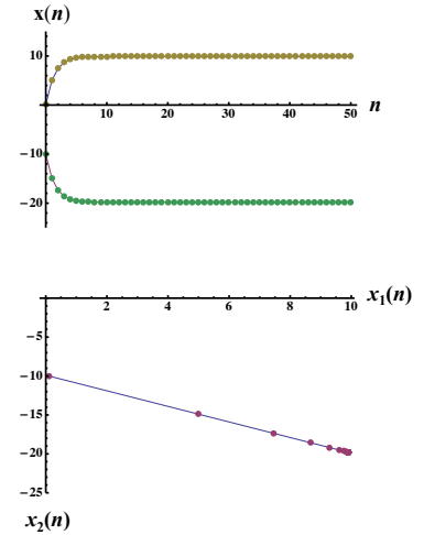
Figure 11.4: Dynamics (top) and phase plot (bottom), for the linear model with \mathbf{A} as in Eq. (11.12), and x_1(0) = 0.1, x_2(0) = -10 . Top: x_1(n) brown and x_2(n) green.
