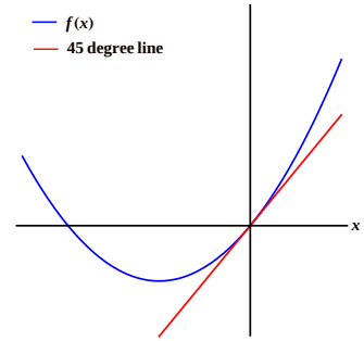
Figure 10.10: Graph of f(x) = x \cdot (1 + b \cdot x) relative to the 'x = y line' when b > 0
