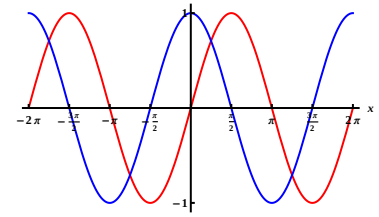
Figure 17.11: Red: \sin(x) , Blue: \cos(x)
