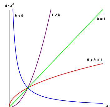
Figure 17.7: The different types of power functions. In all cases a > 0
