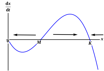
Figure 12.6: Graph of \frac{dx}{dt} versus x for the Allee model. Arrows indicate directions of change in x .
