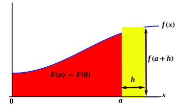
Figure 20.3: A function f(x) with its area under the curve from x = 0 to x = a . Further explanation: see main text.
