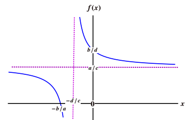
Figure 17.6: Example of the shape of a linear fractional function if ad < cb .
