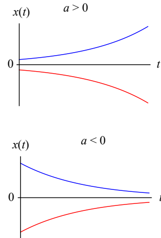
Figure 12.2: Shape of solutions of the linear differential equation in 12.10 for different combinations of a , and initial conditions x(0) > 0 (blue) and x(0) < 0 (red).
