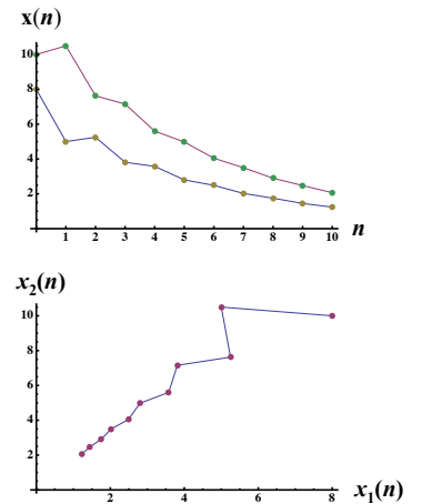
Figure 11.2: Dynamics (top) and phase plot (bottom), for the linear model with \mathbf{A} as in Eq. (11.10), and x_1(0) = 8, x_2(0) = 10 . Top: x_1(n) brown and x_2(n) green.
