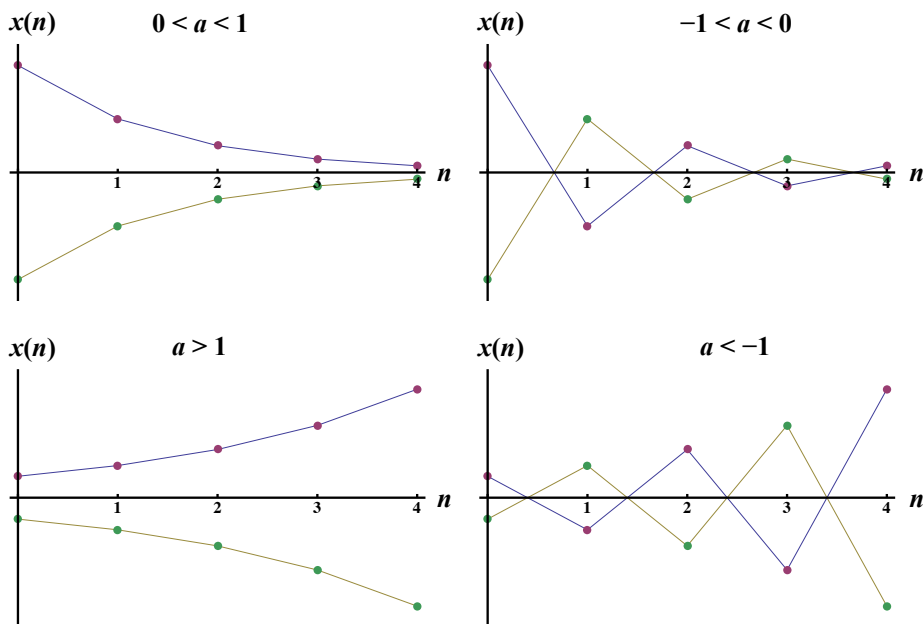
Figure 10.2: Examples of dynamics of the linear model for different ranges of the parameter a .
