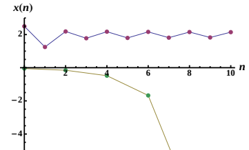
Figure 10.4: Dynamics of the model in Eq. (10.25) for two different initial conditions.
