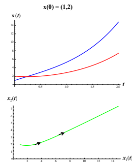
Figure 13.6: Dynamics of the linear model with \mathbf{A} given in (13.28) and an initial condition that leads away from the equilibrium. Top: x_1(t) (blue) and x_2(t) (red) versus time. Bottom: phase plot.
