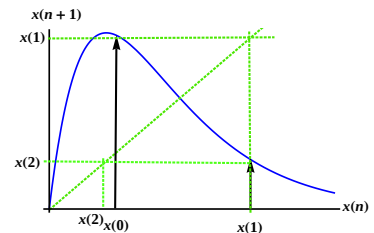
Figure 10.14: Finding the values of x(1) and x(2) from the graph, using the 45° line.
