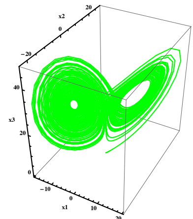
Figure 13.9: Strange attractor of the Lorentz system in (13.57) with a = 10, b = 8/3, c = 28 .
