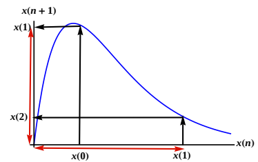
Figure 10.13: Finding the value of x(2) from the graph.
