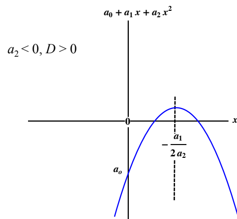
Figure 17.2: The different types of second-degree polynomials.
