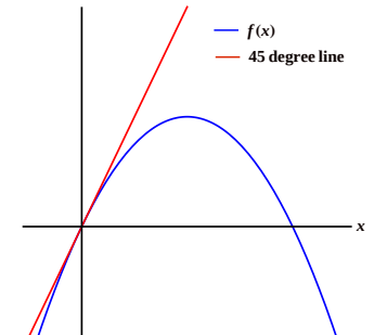
Figure 10.11: Graph of f(x) = x \cdot (1 + b \cdot x) relative to the 'x = y line' when b < 0
