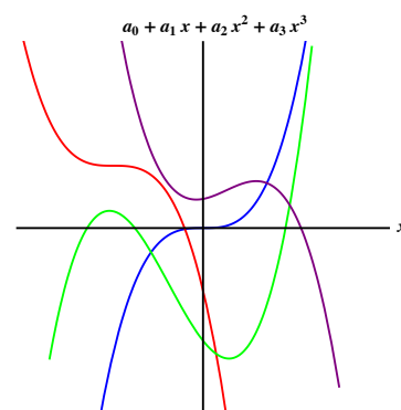
Figure 17.3: Examples of 3rd-degree polynomials.
