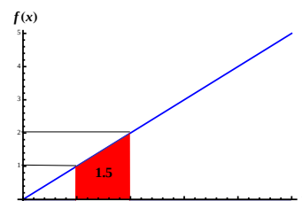
Figure 20.1: The integral from 1 to 2 of the function f(x) = x equals the surface under the function, which is 1.5.
