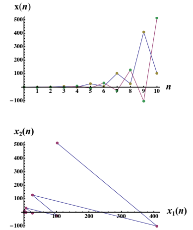
Figure 11.8: Dynamics (top) and phase plot (bottom), for the linear model with \mathbf{A} as in Eq. (11.16), and x_1(0) = 0.1, x_2(0) = 0.5 . Top: x_1(n) brown and x_2(n) green.
