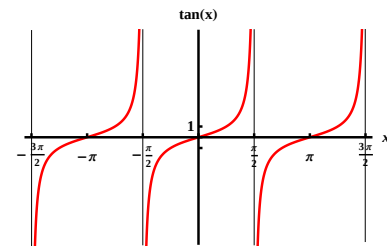
Figure 17.12: \tan(x)
