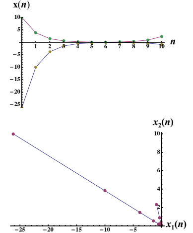
Figure 11.7: Dynamics (top) and phase plot (bottom), for the linear model with \mathbf{A} as in Eq. (11.15), and x_1(0) = -26.18, x_2(0) = 10 . Top: x_1(n) brown and x_2(n) green.
