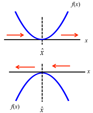
Figure 12.5: Illustration of stability properties of a quadratic model. Blue lines indicate f(x) = b \cdot x^2 , with b > 0 in top figure, and b < 0 in bottom figure. Arrows indicate the directions of change in x .
