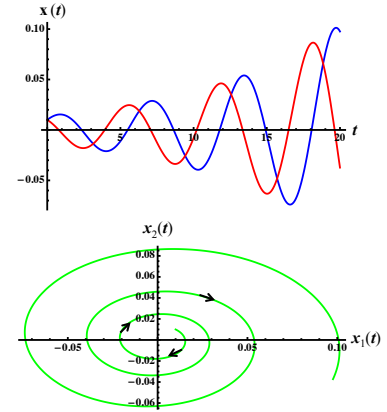
Figure 13.8: Dynamics of the linear model with \mathbf{A} given in (13.30) and initial condition (0.01, 0.01) . Top: x_1(t) (blue) and x_2(t) (red) versus time. Bottom: phase plot.
