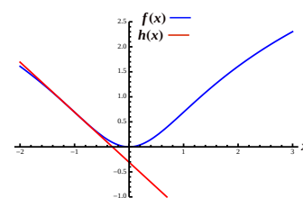
Figure 19.7: Graph of the function in (19.19) and its first order Taylor approximation in the point x = -1 . This is also sometimes called a Taylor expansion around the point a .
