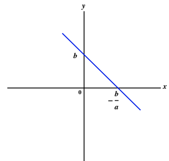
Figure 9.1: the graph of (9.4) when a < 0 and b > 0 .
