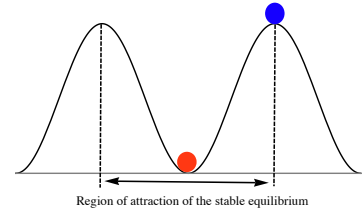
Figure 10.6: Marbles in a landscape, illustrating an unstable equilibrium (blue), and a locally stable equilibrium (red) with its region of attraction.
