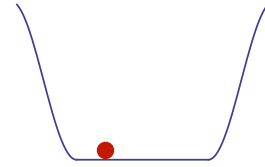
Figure 10.7: A marble in a landscape, at a neutrally stable equilibrium.
