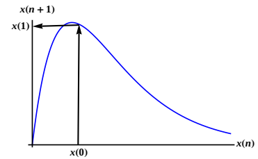
Figure 10.12: Relation between x(n) and x(n+1) for the Ricker model.
