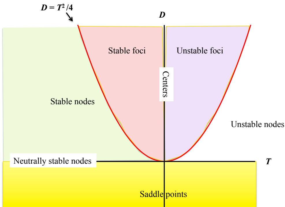
Figure 13.1: Overview of the different types of dynamics of the linear two-dimensional model, for different combinations of D and T . See text below for further explanation.
