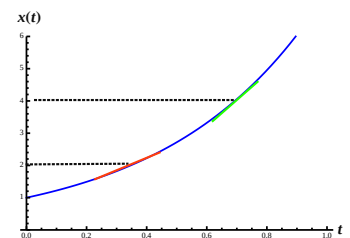
Figure 12.1: An example of the function x(t) corresponding to the differential equation in (12.1). The red line is the tangent to the graph at x = 2 , with slope 4, and the green line is the tangent at x = 4 , with slope 8.
