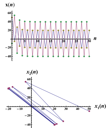
Figure 11.5: Dynamics (top) and phase plot (bottom), for the linear model with \mathbf{A} as in Eq. (11.13), and x_1(0) = 50, x_2(0) = -10 . Top: x_1(n) brown and x_2(n) green.
