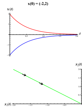
Figure 13.5: Dynamics of the linear model with \mathbf{A} given in (13.28) and an initial condition that leads to the equilibrium. Top: x_1(t) (blue) and x_2(t) (red) versus time. Bottom: phase plot.
