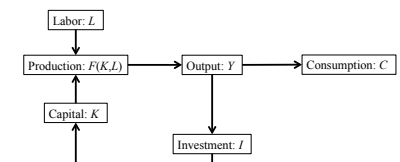
Figure 4.1: Flow diagram of the Solow-Swan model
