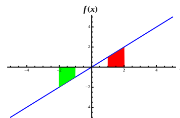
Figure 20.2: The integral from -2 to -1 of the function f(x) = x equals minus the surface between the function and the horizontal axis. Since the surfaces of the green and red areas are the same, the integral equals -1.5 .
