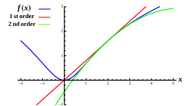
Figure 19.8: Graph of the function in (19.19), with its first(red)- and second order (green) Taylor approximation in the point x = 2 .
