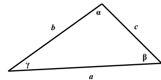
Figure 17.13: Definition of symbols used in the sine- and cosine rules.
