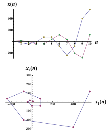
Figure 11.9: Dynamics (top) and phase plot (bottom), for the linear model with \mathbf{A} as in Eq. (11.11), and x_1(0) = 10, x_2(0) = 10 . Top: x_1(n) brown and x_2(n) green.
