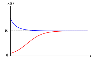
Figure 12.3: Shape of solutions of the logistic model in (12.6), for x(0) < K (red) and x(0) > K (blue).
