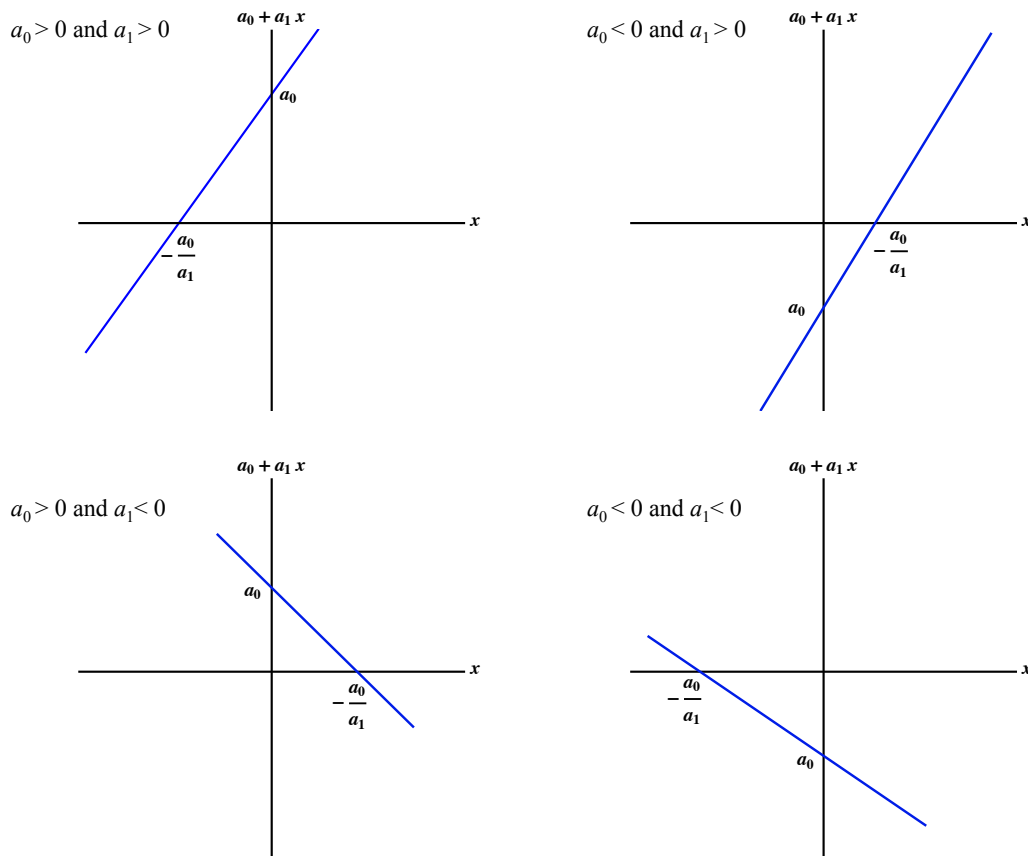
Figure 17.1: The different types of first-degree polynomials.
