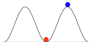
Figure 10.5: Marbles in a hilly landscape with two equilibria: red at a stable equilibrium, blue at an unstable equilibrium.
