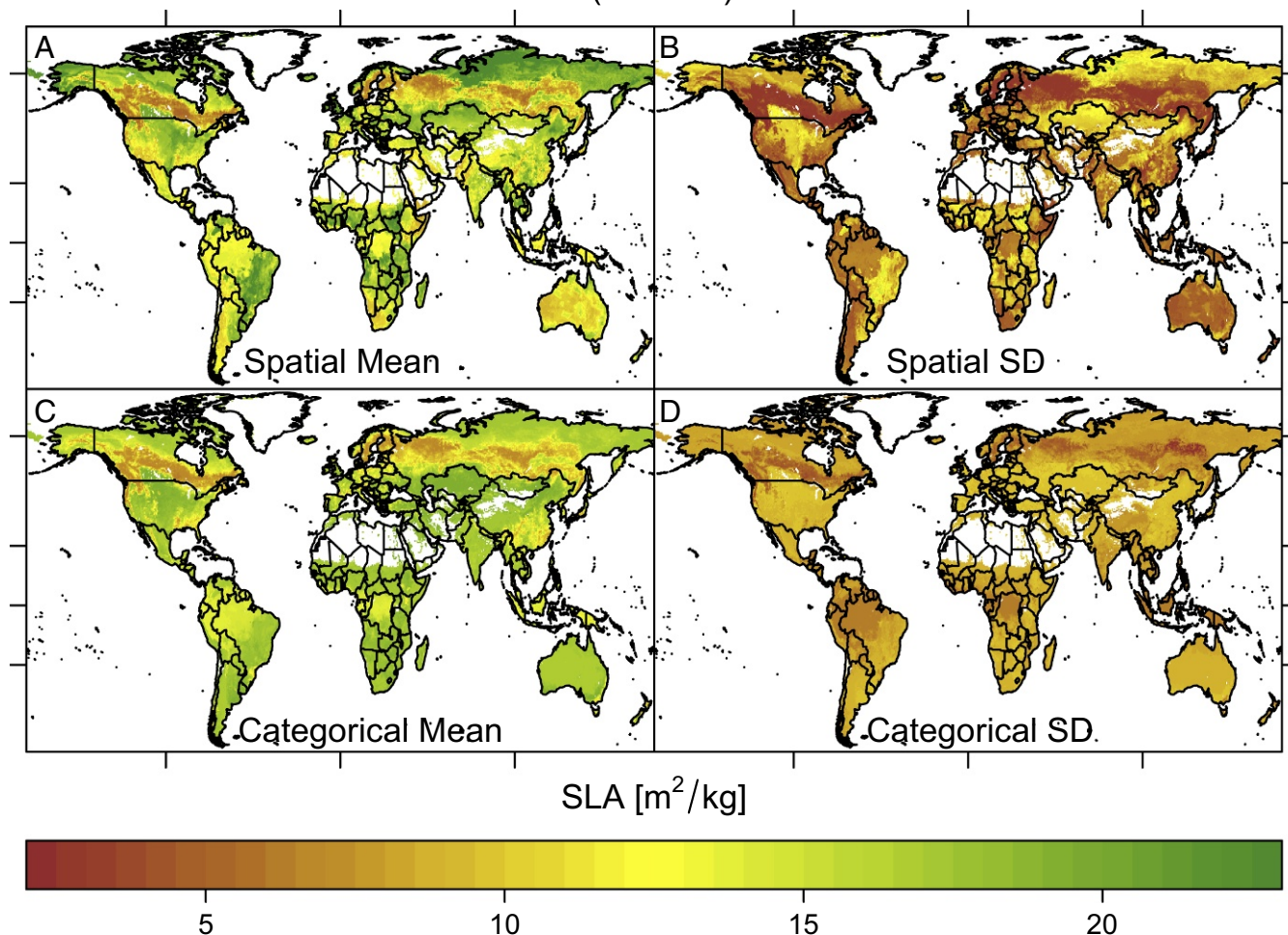
Fig. 2. SLA maps. (A and B) Narrow (14-PFT) Bayesian spatial model pixel mean and SD estimates, respectively. (C and D) Narrow (14-PFT) categorical model pixel mean estimates and SD estimates, respectively. For clarity, the color bars have been truncated at the compound 5th and 95th percentiles of both models. Latitude tick marks indicate the equator, tropics, and Arctic Circle and longitude is marked at 100^\circ\text{W} , 0^\circ , and 100^\circ\text{E} .
