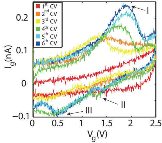
Figure 3: Plots showing 6 CV scans. The first cyclic voltammogram does not show any peaks and indicates a chemically pure IL, while the others show peaks increasing in amplitude as a function of the cycle number. As the number of CV scans increases, several peaks (I, II and III) start to appear. Peak I is located between 1.35 and 1.95 V and indicates an initial reduction. Peak II and III are located between 1.1 and 1.435 V, and 0.29 and 0.55 V, respectively. We observe that the potential separation between peaks I and II is 0.27 < \Delta V < 0.51 V. Furthermore, the amplitude of peak I is a factor 3 to 10 higher than that of peaks II and III.
