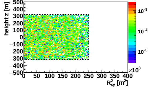
(d) Positions of tauCCshow events after other selection criteria.
