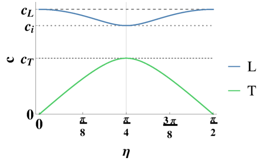
FIG. 13. Velocities of the massless modes in the columnar phase as a function of interrogation angle \eta from Eq. (193). Here we have chosen a representative value of the Poisson ratio \nu = 0.3 . The velocity of the longitudinal mode varies from that of the longitudinal phonon c_L at \eta = 0, \pi/2 while it is reduced to c_i = \sqrt{c_L^2 - c_T^2} at \eta = \pi/4 . The velocity of the transverse mode is maximal at \eta = \pi/4 where it reaches that of the transverse phonon c_T , while it is reduced to zero at \eta = 0, \pi/2 , where it also has vanishing pole strength. This pattern is identical to that of the 2D smectic [42].
