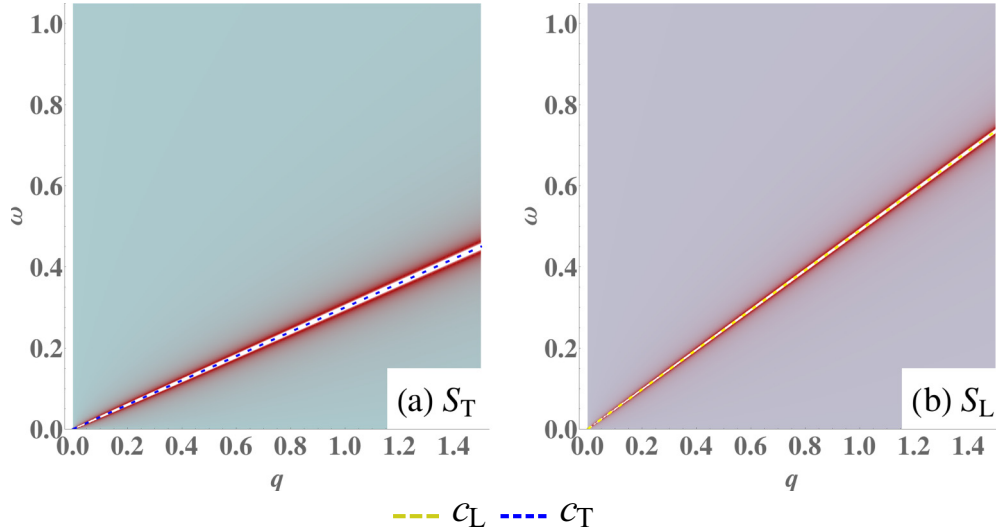
FIG. 6. Spectral functions Eq. (97) (left: transverse; right: longitudinal) of the isotropic solid in units of the inverse shear modulus 1/\mu \equiv 1 , with Poisson ratio \nu = 0.2 . The width of the poles is artificial and denotes the relative pole strengths: these ideal poles are actually infinitely sharp. The propagating modes, phonons, are massless (zero energy as q \rightarrow 0 ) and have linear dispersion \omega = cq . The velocities are transverse c_T and longitudinal c_L respectively. The pole in the transverse sector is doubly degenerate as there are two transverse phonons.
