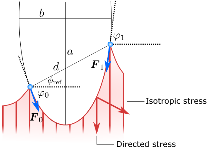
Figure 5.1: Schematic depiction of a part of a cell. The cell edge (curved red line) is fixed in adhesions (blue points) to the membrane. In between these points, the membrane assumes the shape of part of an ellipse (black). The long axis a of the ellipse is aligned with the stress fibers (red) inside the cell. The forces \vec{F}_0 and \vec{F}_1 (blue arrows) are ordered counter-clockwise on the edge and are tangent to the ellipse. Angles between the tangents at the locations of the forces and the ellipse are labeled \phi_0 and \phi_1 . The angle between the line (length d ) connecting the forces and the short axis b of the ellipse is \phi_{\text{ref}} .
