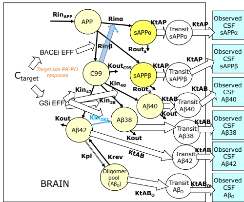
Figure 8.6: \beta - \gamma -O-APP model (Chpt. 7). The model comprised fourteen compartments: Eight biomarker compartments in brain (yellow circles) and six transit compartments from brain to CSF (white circles). Six biomarkers were measured in CSF (sAPP \alpha , sAPP \beta , A \beta 40, A \beta 42, A \beta 38 and A \beta O), indicated by the blue boxes. The drug effect of the BACE1 inhibitor (BACEi EFF) inhibited Rin\beta . The drug effect of the GS inhibitor (GSi EFF) inhibited Kin_{40} , Kin_{40} , Kin_{38} and Kin_{382} . The tick blue arrow indicates the homeostatic feedback on \alpha -secretase through the action of C99. Model extensions compared to the \beta -O-APP model are indicated in blue.
