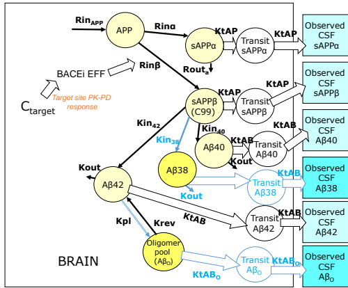
Figure 8.5: \beta -O-APP model (Chpt. 6). The model comprised thirteen compartments: Seven biomarker compartments in brain (yellow circles) and six transit compartments from brain to CSF (white circles). Six biomarkers were measured in CSF (sAPP \alpha , sAPP \beta , A \beta 40, A \beta 42, A \beta 38 and A \beta O), indicated by the blue boxes. The drug effect of the BACE1 inhibitor (EFF) inhibited Rin\beta . sAPP \beta was used in the model structure as a surrogate substrate for C99 in the \gamma -secretase cleavage step. Model extensions compared to the \beta -APP model are indicated in blue.
